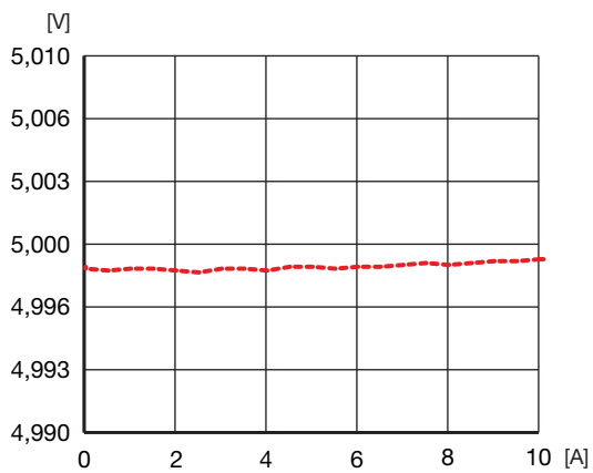
Output voltage vs. load current at T_{Pcb}=+25\text{ }^{\circ}\text{C} , V_{in}=27\text{ V} .
