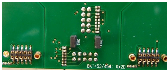
Figure 3.4 Factory default jumper settings of ROA 128 3835
