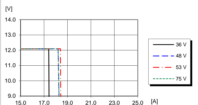
Output voltage vs. load current at I_O > I_{Omax} , T_{P1} = +25^{\circ}\text{C} .
