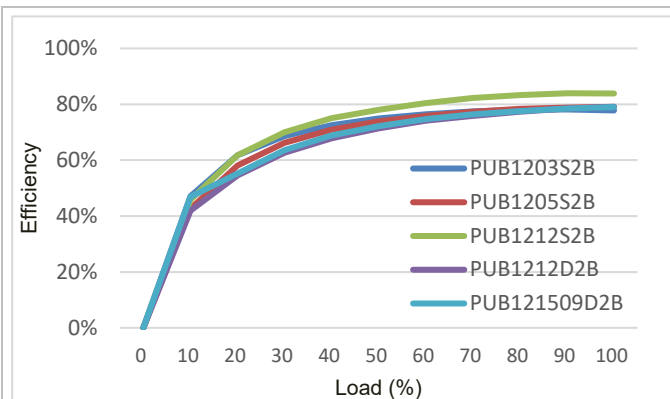
PUB12-2B Efficiency vs. load current at T_{P1} = +25^{\circ}\text{C} .
