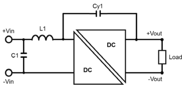
Test set-up
