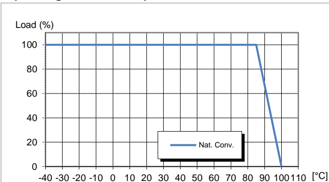
PUA03-1A, PUA05-1A, PUA12-1A Available load vs. ambient air temperature. See Thermal Consideration section.
