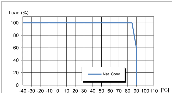
PUA24-1A Available load vs. ambient air temperature. See Thermal Consideration section.
