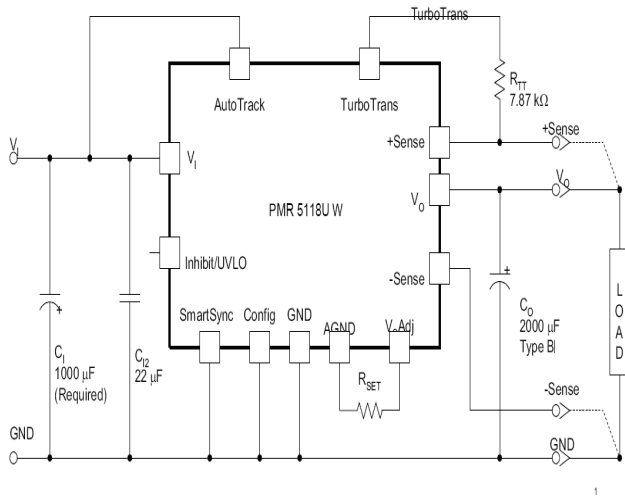
Figure: Typical TurboTrans™ Application
