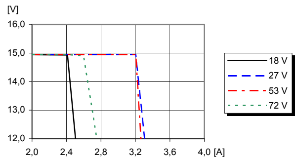
Output voltage vs. load current at I_O > \max I_O , T_{P1} = +25^{\circ}\text{C} The module enters hiccup mode when the output current exceeds current limit.
