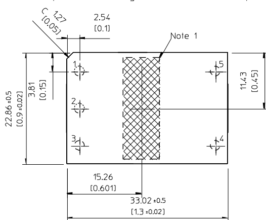
Pin positions according to the recommended footprint
