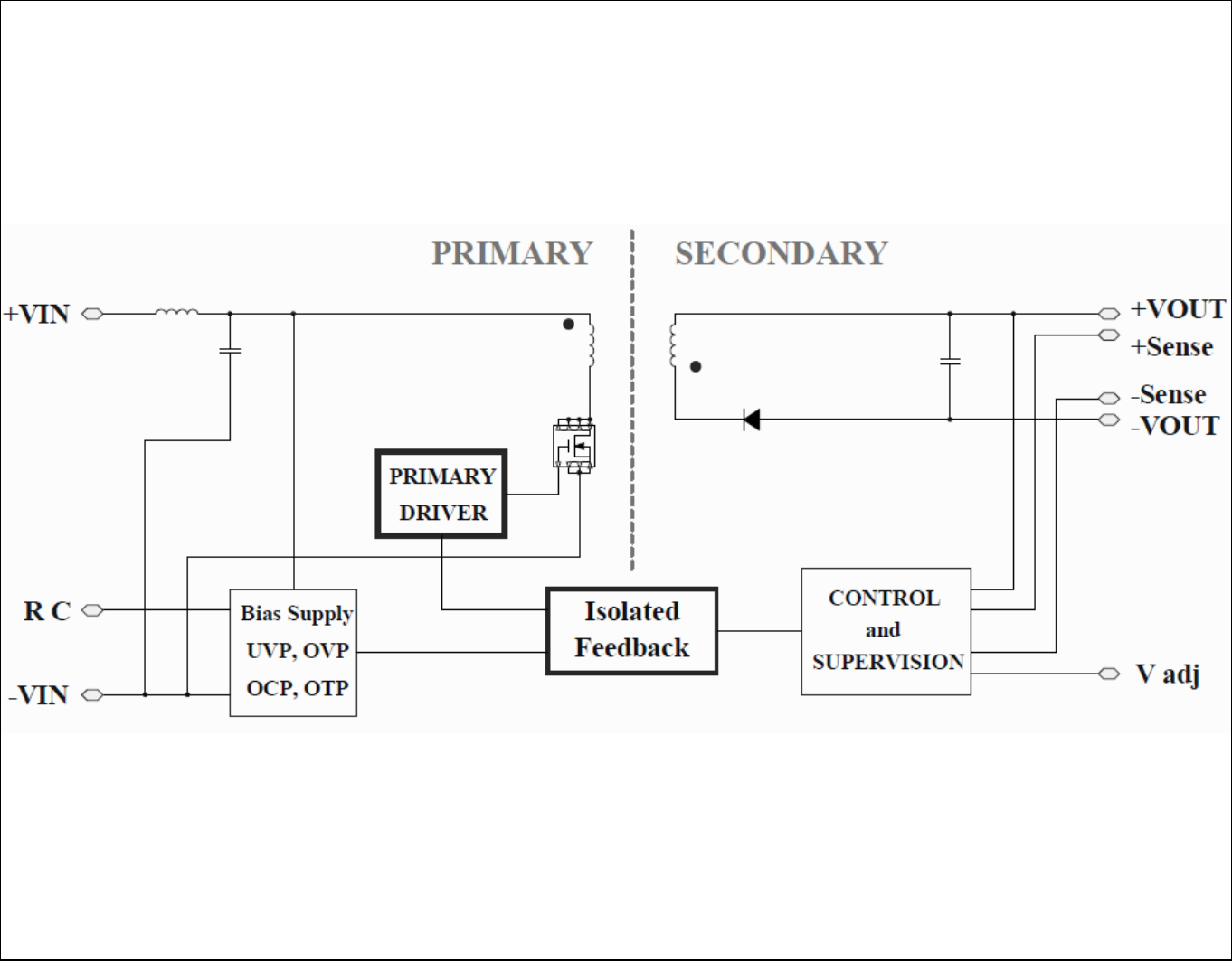
Fundamental Circuit Diagram For PKM7516ZWPI(P), PKM7516JWPI(P), PKM7516HWPI(P)
