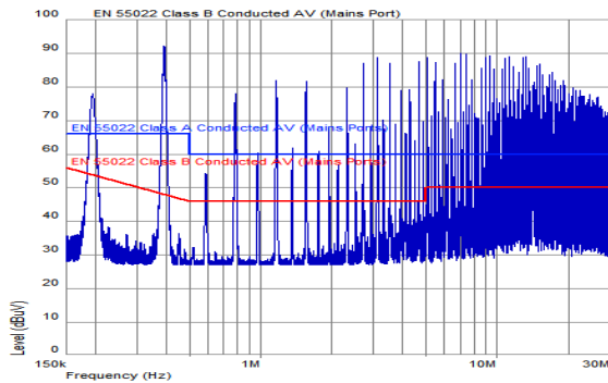
EMI without filter (1 x PKM 4817LNH PI)
