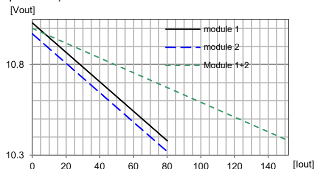
Typical output current from two products with 60mV output voltage initial setting tolerances.
