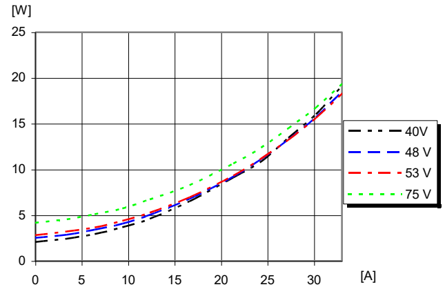
Dissipated power vs. load current and input voltage at T_{P1} = +25^{\circ}\text{C}
