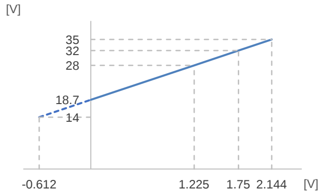
Desired output voltage vs. adjust voltage, R_{adj} = 1 \text{ k}\Omega
