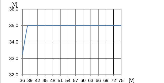
Max adjustable output voltage vs. input voltage at T_{P1} = +25^\circ\text{C} . Max adjustable output voltage \geq 33\text{V} at V_{in}=36\text{V} , P_o=700\text{W}
