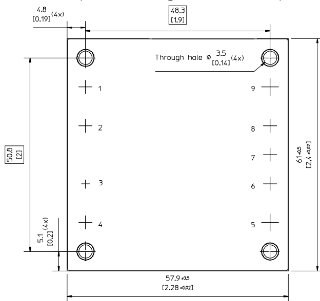
RECOMMENDED FOOTPRINT - TOP VIEW
