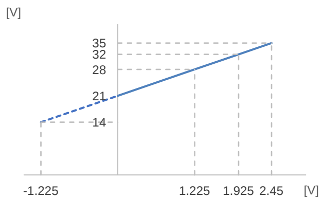
Desired output voltage vs. adjust voltage, R_{adj} = 2 \text{ k}\Omega
