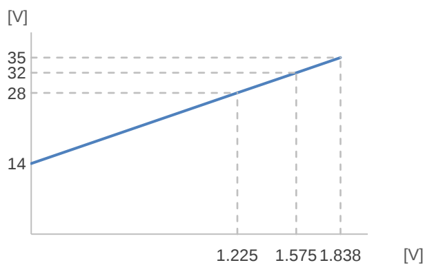
Desired output voltage vs. adjust voltage, R_{adj} = 0 \text{ k}\Omega
