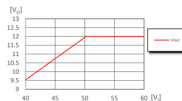
Output voltage vs. input voltage at T_{P1} = +90^{\circ}\text{C}
