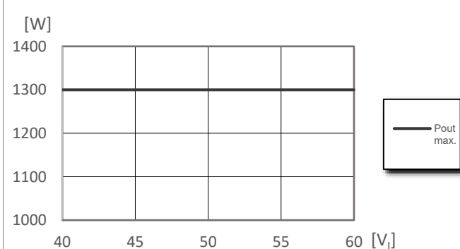
Available output power vs. input voltage, T_{P1} = +90^{\circ}\text{C} V_i 40-46V, T > 180\text{sec} P_O derates by 10%.
