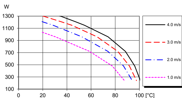
Available output power vs. ambient air temperature and airflow. See Thermal Consideration section.
