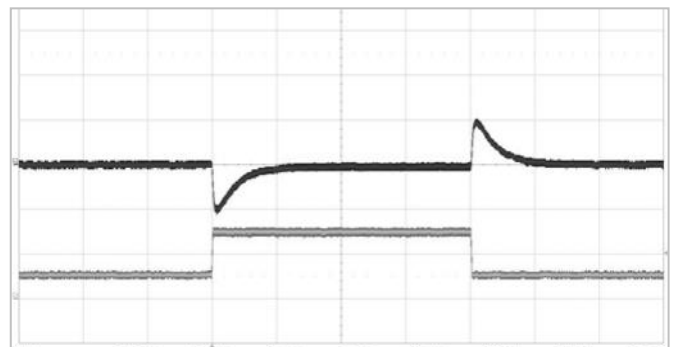
Output voltage response to output current change (10-30-10 A) at V_I = 12\text{ V} , C_O = 8 \times 100\text{ }\mu\text{F} ceramic + 4 \times 470\text{ }\mu\text{F} POSCAP (ESR 10 m \Omega ), T_{PI} = +25^\circ\text{C} , di/dt = 2\text{ A}/\mu\text{s} .
