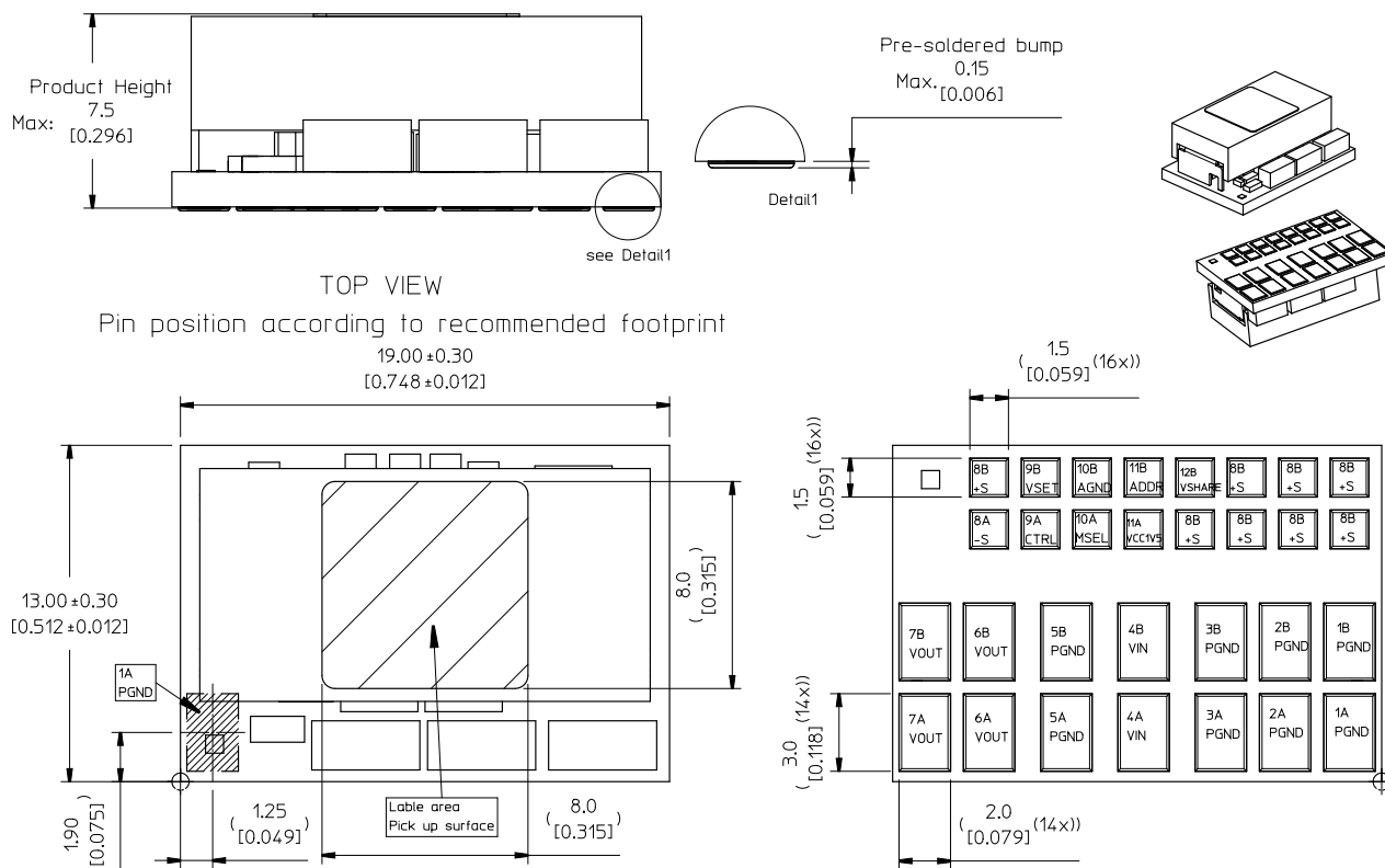
RECOMMENDED FOOTPRINT - TOP VIEW
