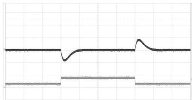
Output voltage response to output current change (5-15-5 A) at V_I=12\text{ V} , C_o=5 \times 100\text{ μF ceramic} + 4 \times 470\text{ μF POSCAP (ESR } 10\text{ mΩ)} , T_{PI} = +25^{\circ}\text{C} , di/dt=2\text{ A/μs} .
