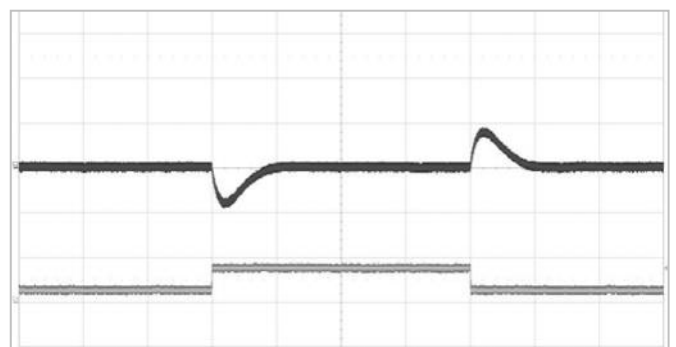
Output voltage response to output current change (5-15-5 A) at V_I=12\text{V} , C_o=8 \times 100\text{ }\mu\text{F} ceramic + 4 \times 470\text{ }\mu\text{F} POSCAP (ESR 10 m \Omega ), T_{PI} = +25^\circ\text{C} , di/dt=2\text{A}/\mu\text{s} .
