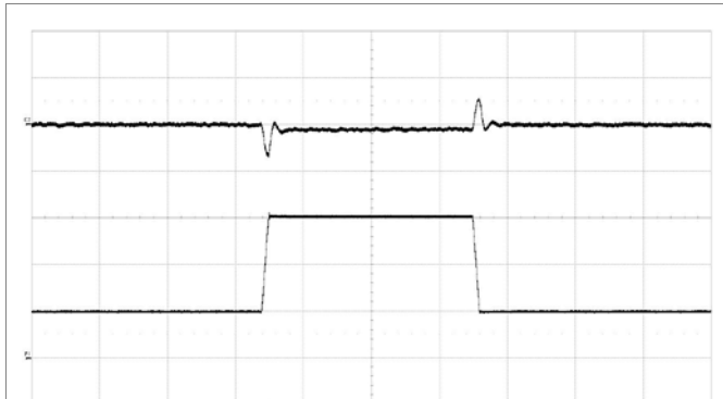
Output voltage response to load current step change (25%–75%–25%) at V_I = 12 V, C_{OUT} = 8 \times 330 \mu F / 10 m\Omega + 20 \times 100 \mu F , di/dt = 2 A/µs, ACSR Gian=219 and ASCR Residual=82. Scale from top: 50 mV/div, 20 A/div, 200 µs/div. Note: Sense pins are connected to load.
