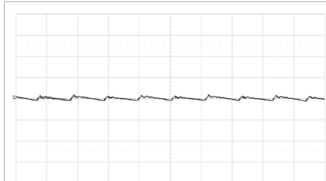
Fundamental output voltage ripple at V_I = 12 V, I_O = 80 A, C_{OUT} = 8 \times 330 \mu F / 10 m\Omega + 20 \times 100 \mu F Scale: 10 mV/div, 1 µs/div, 20 MHz bandwidth. See section Output Ripple and Noise.
