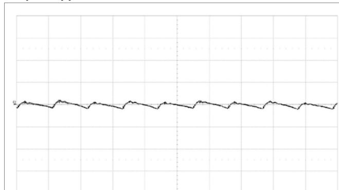
Fundamental output voltage ripple at V_I = 12\text{ V} , I_O = 80\text{ A} , C_{OUT} = 8 \times 330\text{ }\mu\text{F}/10\text{ m}\Omega + 20 \times 100\text{ }\mu\text{F} . Scale: 10 mV/div, 1 \mu\text{s}/\text{div} , 20 MHz bandwidth. See section Output Ripple and Noise.
