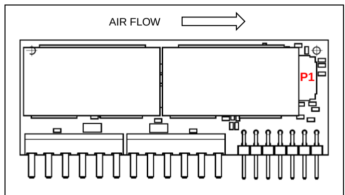
Temperature positions and air flow direction (side view).
