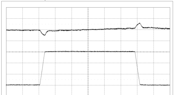
Output voltage response to load current step change (30–90–30 A) at V_i = 12\text{ V} , C_{OUT} = 10 \times 470\text{ }\mu\text{F}/5\text{ m}\Omega + 10 \times 100\text{ }\mu\text{F} , di/dt = 2\text{ A}/\mu\text{s} , ASCR Gain = 300 and ASCR Residual = 90. Scale from top: 50 mV/div, 20 A/div, 100 \mu\text{s} /div. Note: Sense pins are connected to load.
