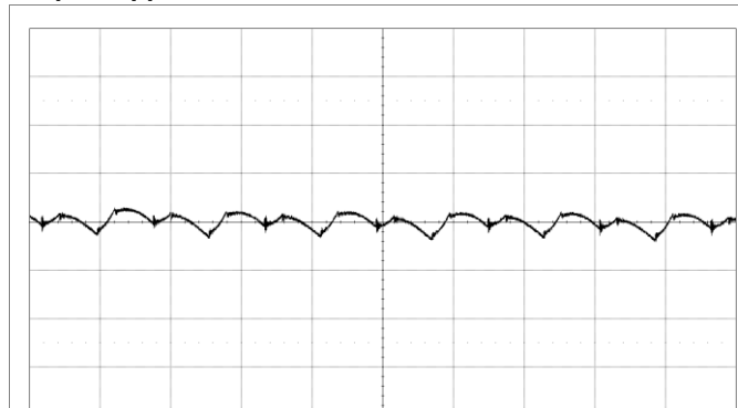
Fundamental output voltage ripple at V_i = 12\text{ V} , I_o = \text{max } I_o , C_{OUT} = 10 \times 470\text{ }\mu\text{F}/5\text{ m}\Omega + 10 \times 100\text{ }\mu\text{F} . Scale: 10 mV/div, 2 \mu\text{s} /div, 20 MHz bandwidth. See section Output Ripple and Noise.
