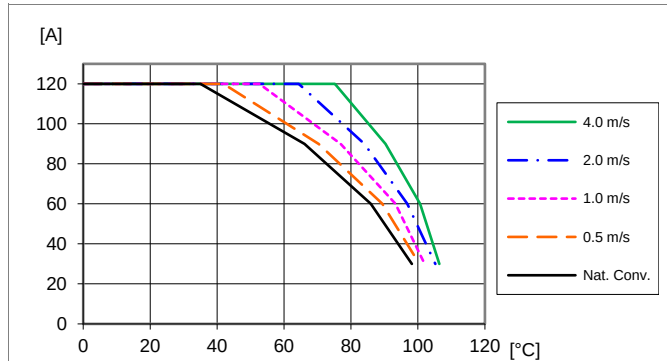
Available load current vs. ambient air temperature and airflow at V_i = 12 V.
