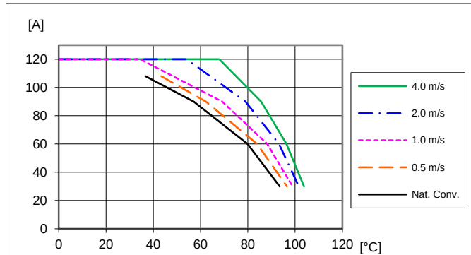
Available load current vs. ambient air temperature and airflow at V_i = 12\text{ V} .
