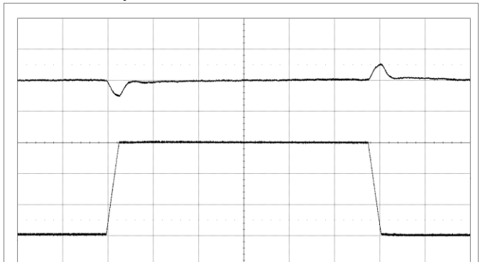
Output voltage response to load current step change (30–90–30 A) at V_i = 12 V, C_{OUT} = 10 \times 470 \mu\text{F}/5 \text{ m}\Omega + 10 \times 100 \mu\text{F} , di/dt = 2 \text{ A}/\mu\text{s} , ASCR Gain = 300 and ASCR Residual = 90. Scale from top: 50 mV/div, 20 A/div, 100 \mu\text{s} /div. Note: Sense pins are connected to load.
