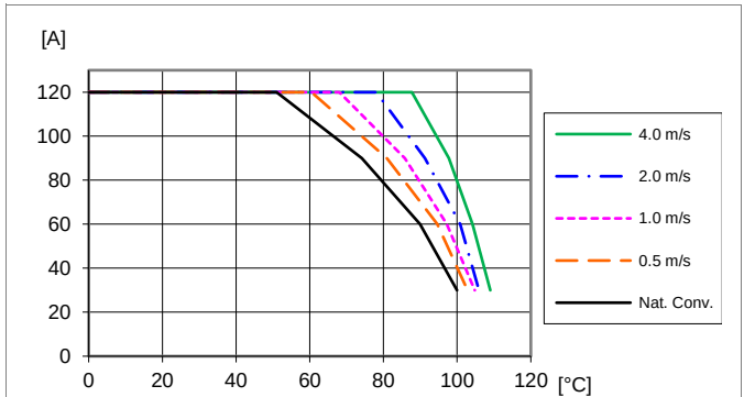
Available load current vs. ambient air temperature and airflow at V_i = 12 V.
