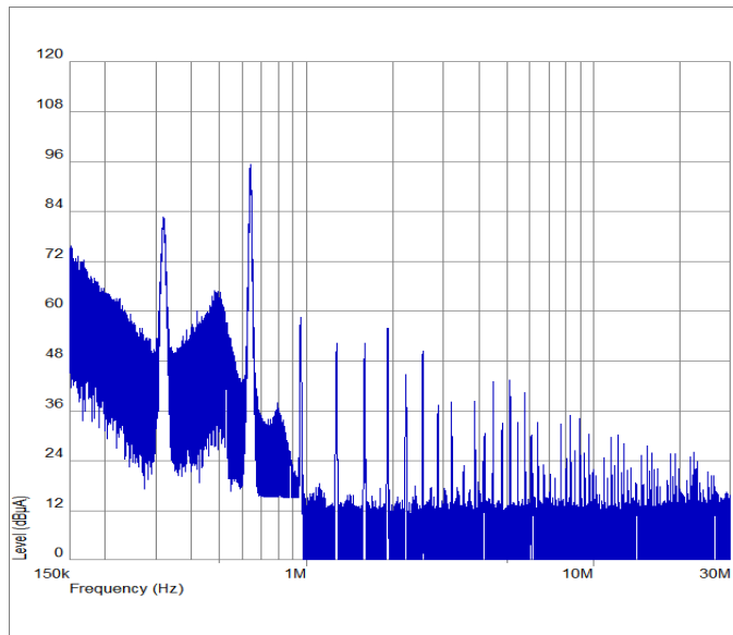
EMI without filter
