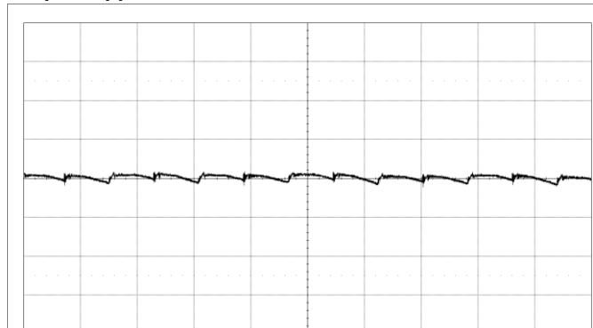
Fundamental output voltage ripple at V_I = 12 V, I_o = \text{max } I_o , C_{OUT} = 10 \times 470 \mu\text{F}/5 \text{ m}\Omega + 10 \times 100 \mu\text{F} . Scale: 10 mV/div, 2 \mu\text{s} /div, 20 MHz bandwidth. See section Output Ripple and Noise.
