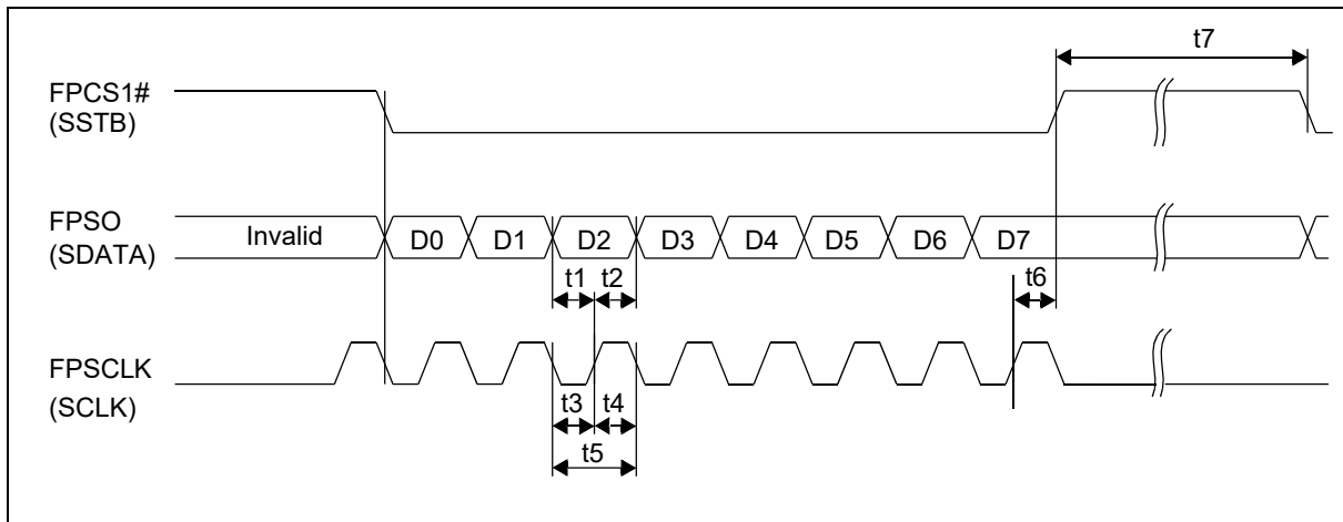
Figure 7-43: LCD1 a-Si TFT Serial Interface Timing
