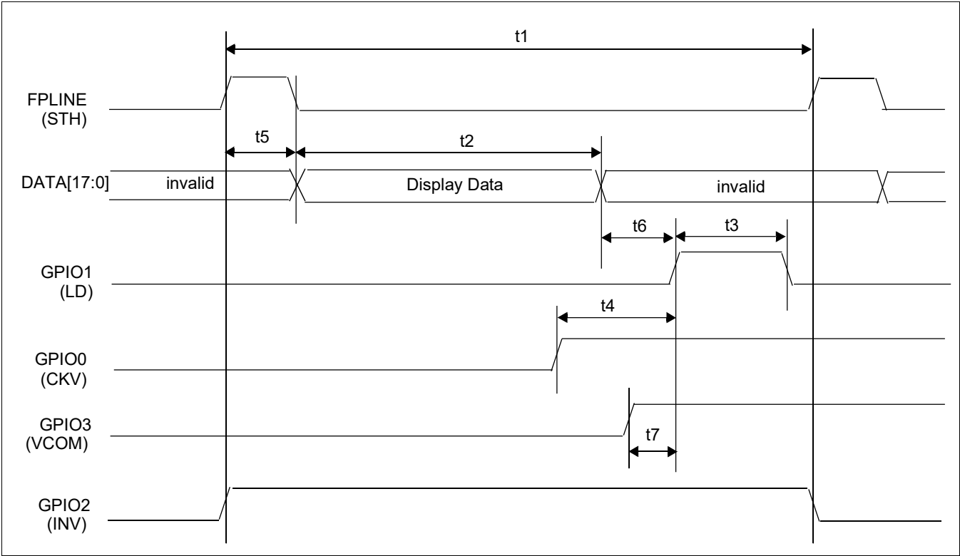
Figure 7-37: α-TFT Panel Horizontal Timing
