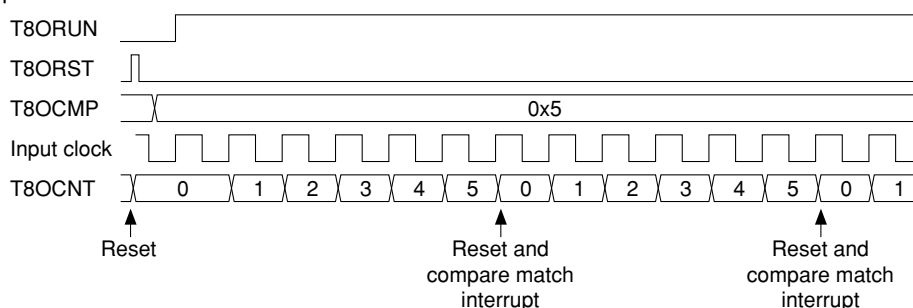
Figure 14.6.1 Basic Operation Timing of Counter
