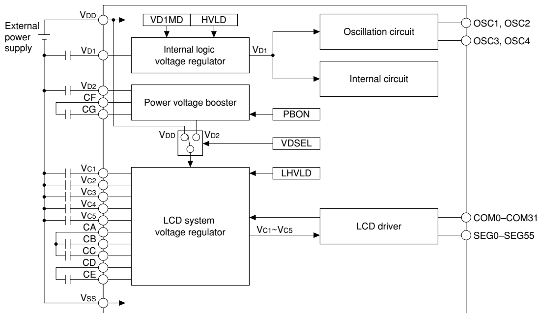
Figure 4.2.1 Configuration of Power Supply Circuit
