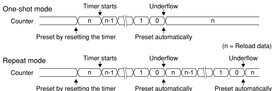
Figure 12.4.1 Preset Timing
