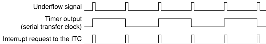
Figure 12.7.1 Timer Output Clock
