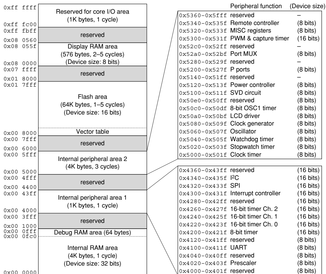
Figure 3.1 S1C17704 Memory Map
