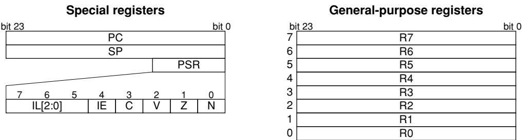
Figure 2.2.1 Registers
