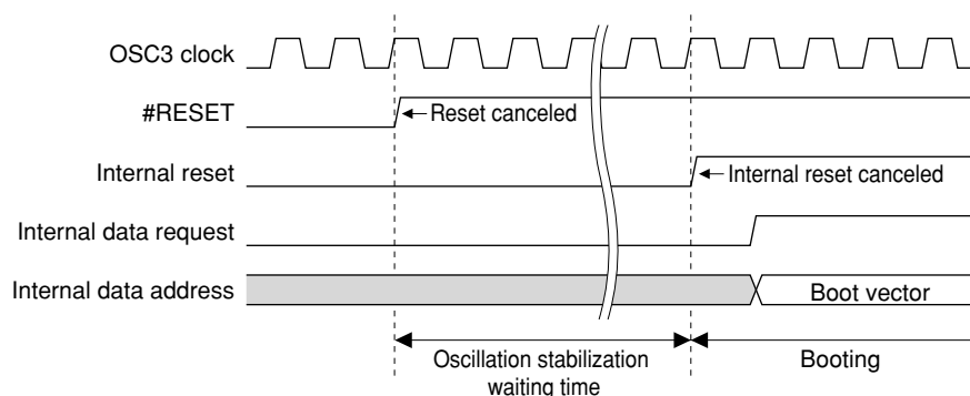
Figure 5.2.1 Operation Sequence Following Cancellation of Initial Reset
