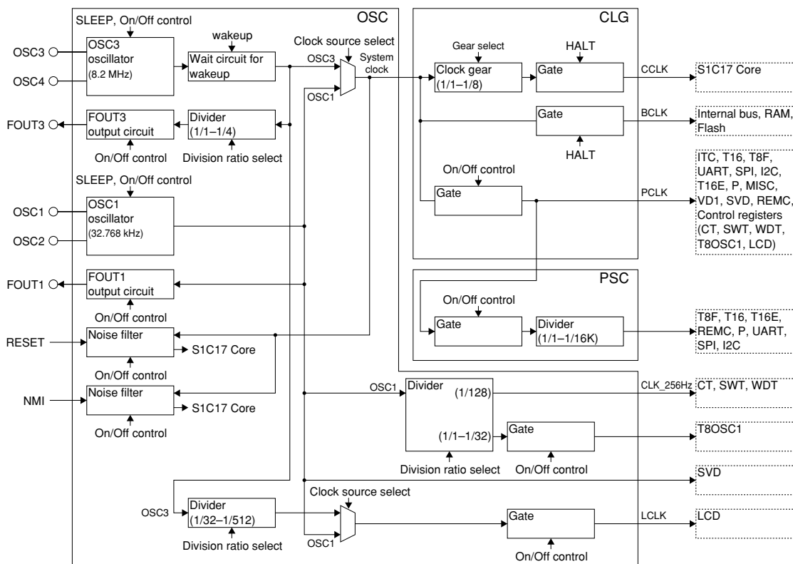
Figure C.1.1 Clock System
