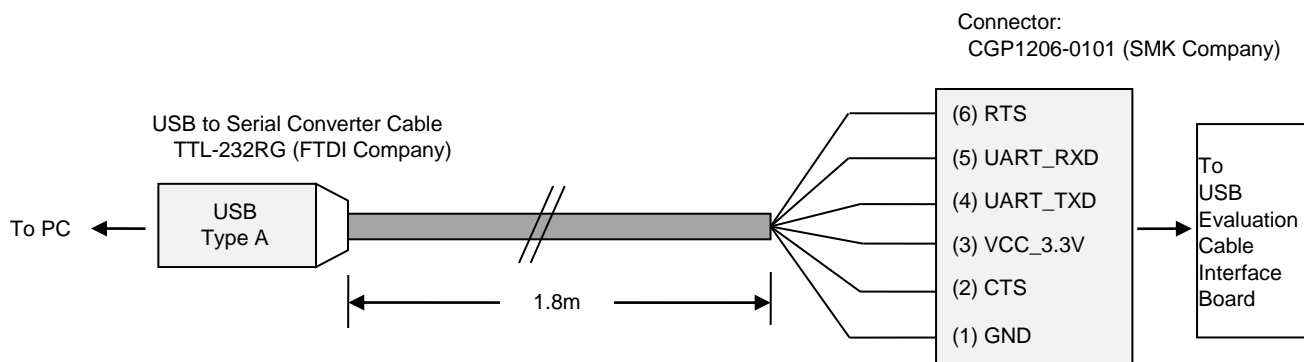
Fig2. Cable Diagram
