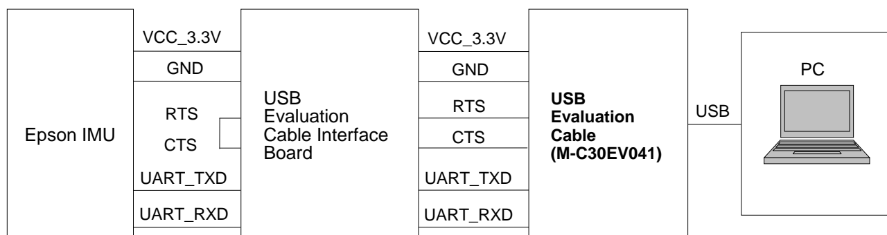
Fig1. Block Diagram
