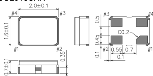
SG2016CAN
