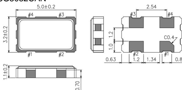
SG5032CAN
