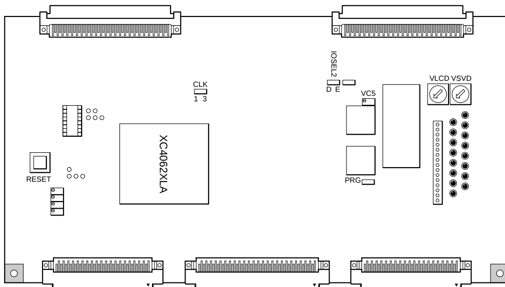
Fig. 1.3.1 External view of S5U1C63000P
