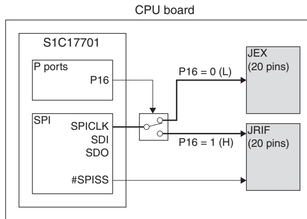
Figure 12.4.1 SPI Port Connector Select Circuit
