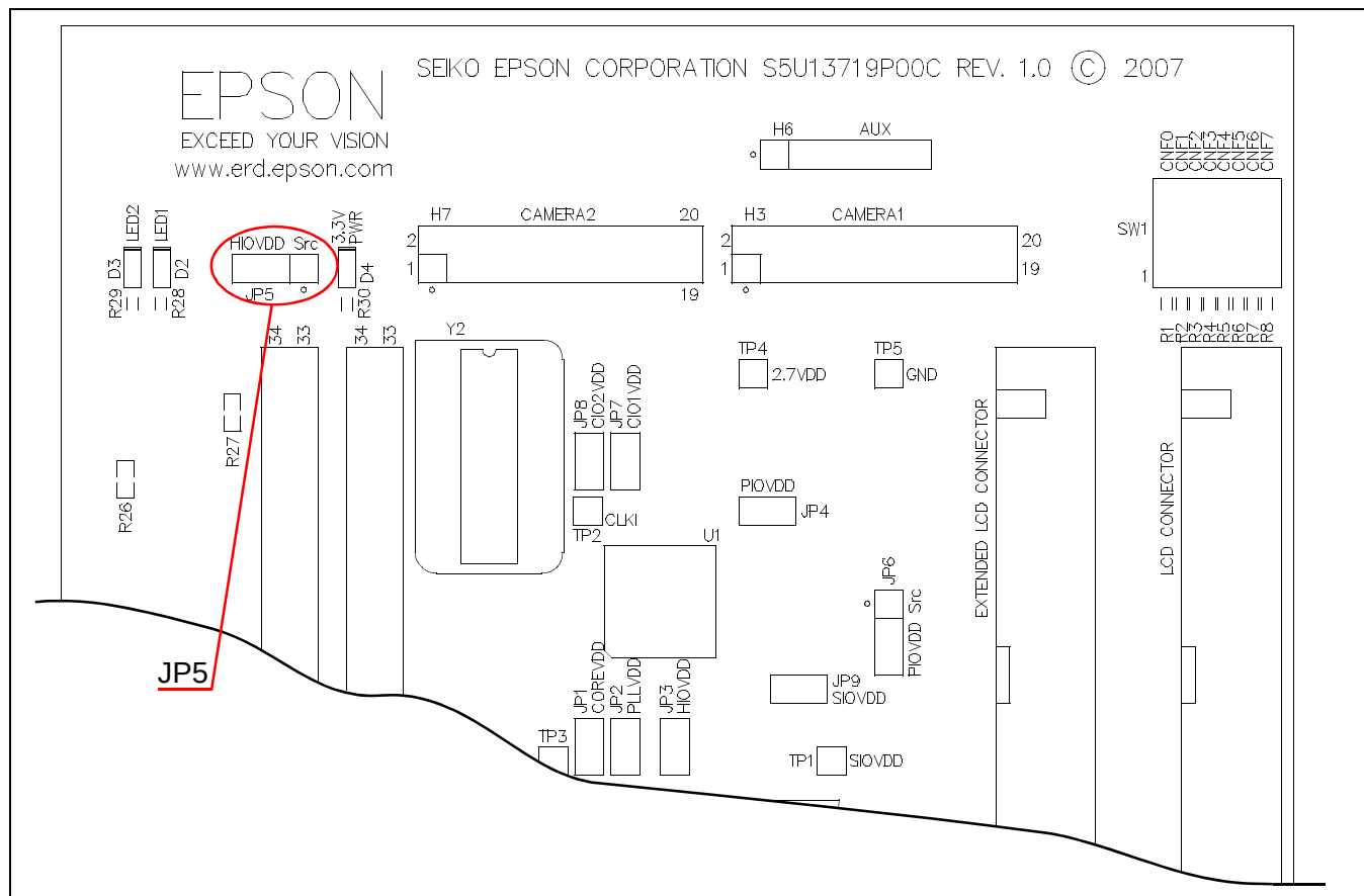
Figure 3-3: Configuration Jumper Location (JP5)
