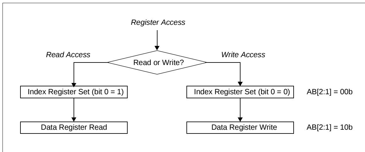
Figure 19-3: Register Access
