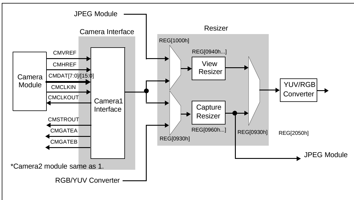
Figure 21-1: Camera Interface
