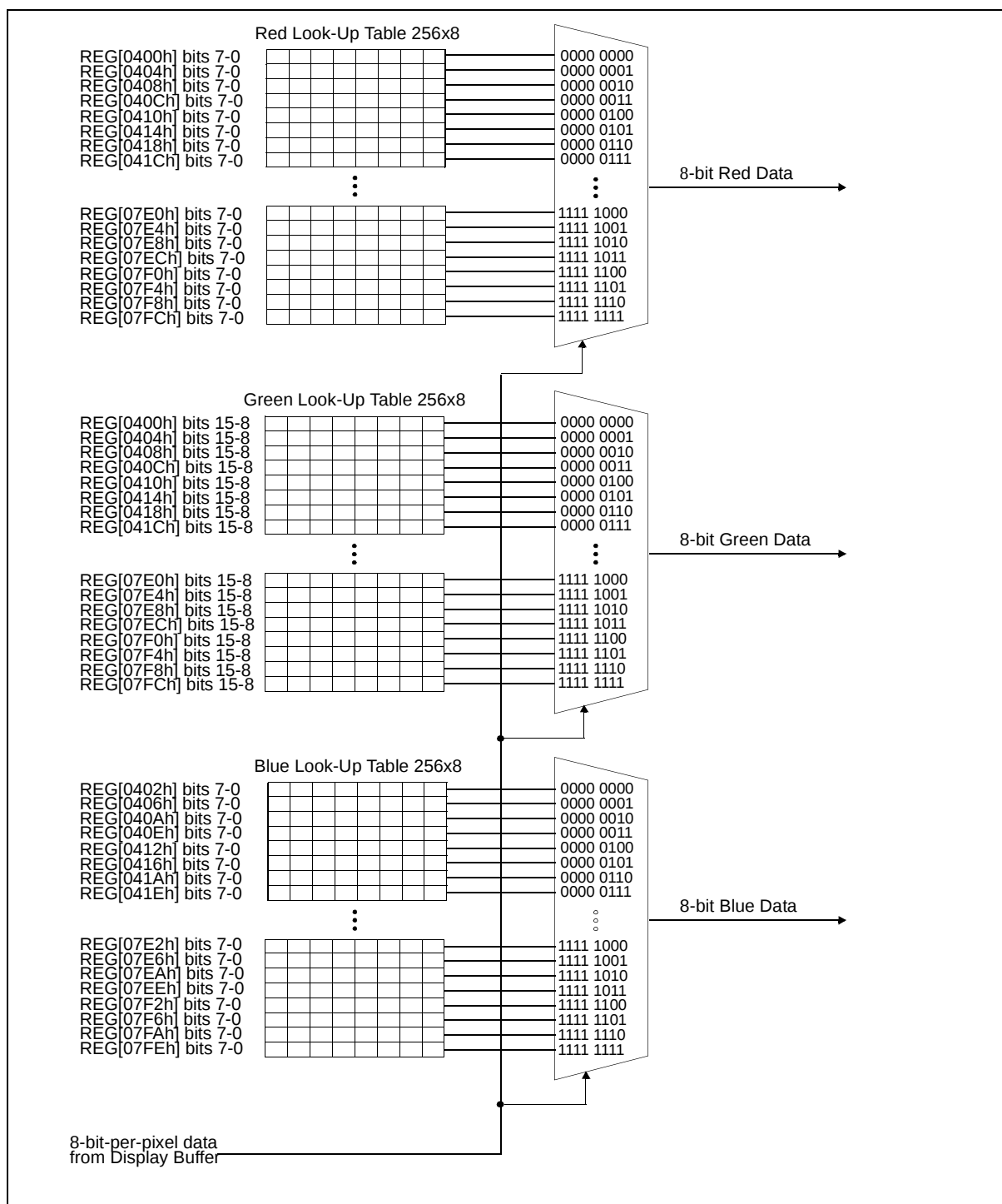
Figure 12-1: LUT1 (8 bpp) Architecture
