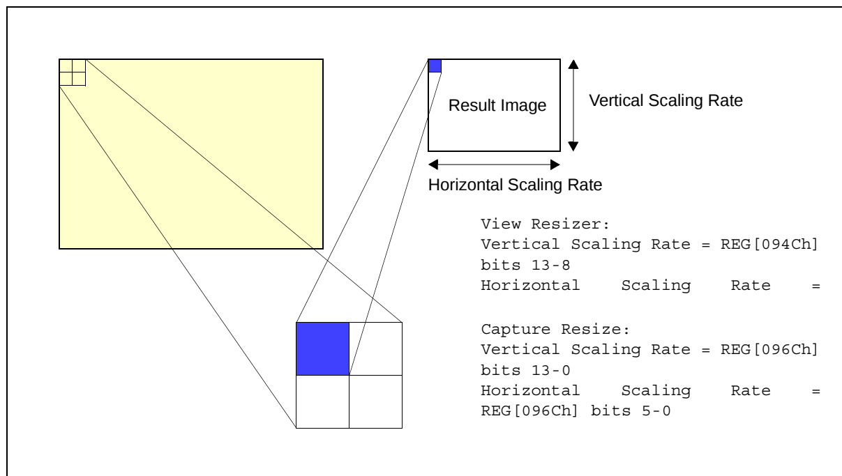
Figure 15-3: Scaling Function
