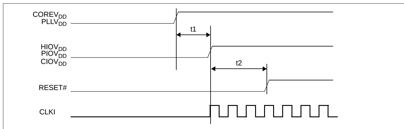
Figure 7-4: Power-On Sequence
