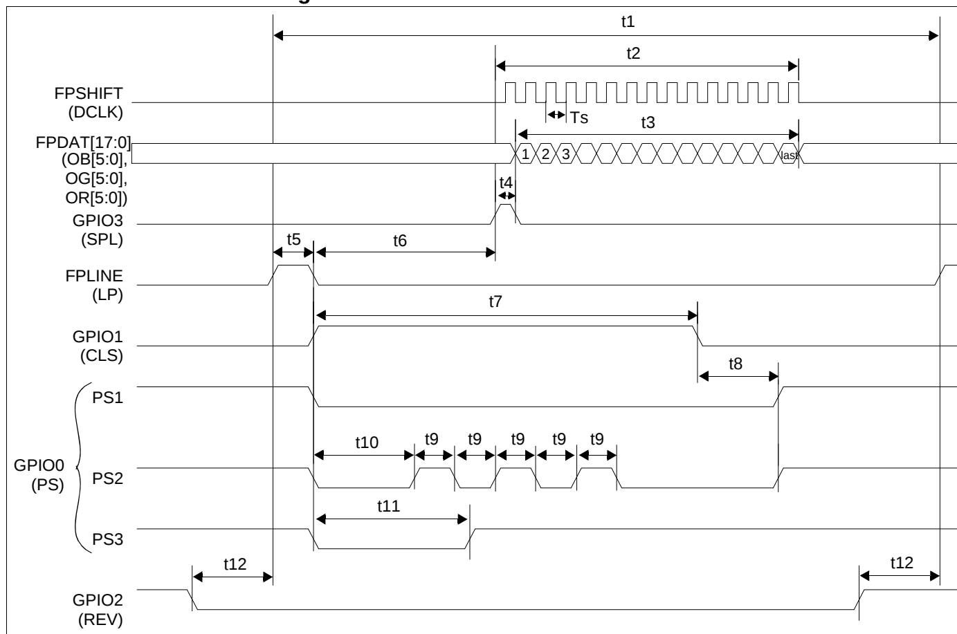
Figure 7-27: HR-TFT Panel Horizontal Timing
