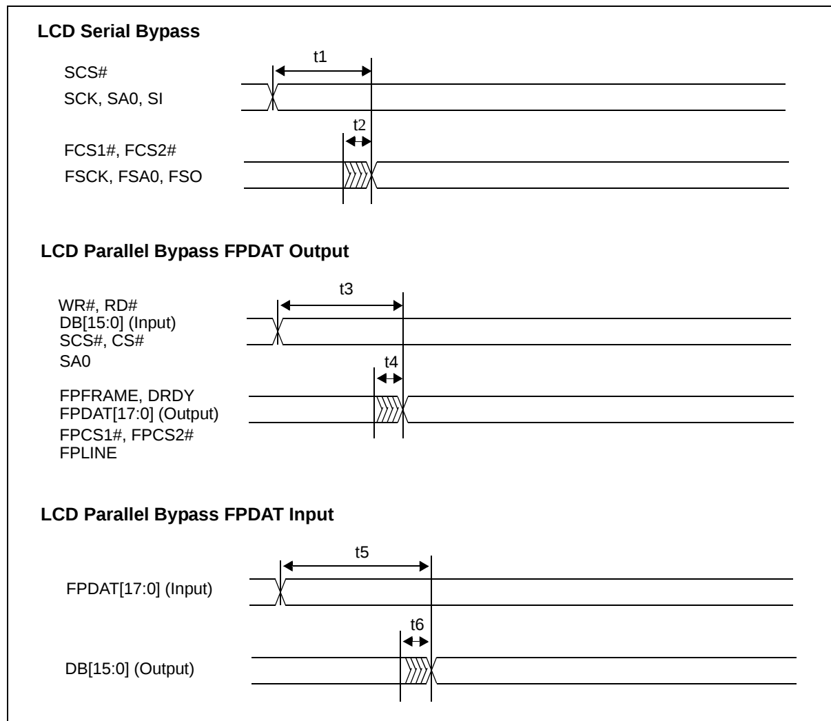
Figure 7-22: LCD Bypass Mode Timing
