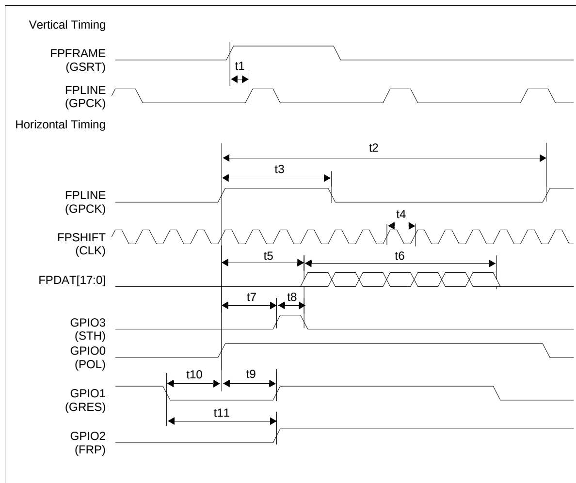
Figure 7-29: Casio TFT Horizontal Timing
