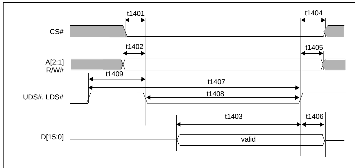
Figure 7-20: Indirect 68 Interface Write Cycle Timing
