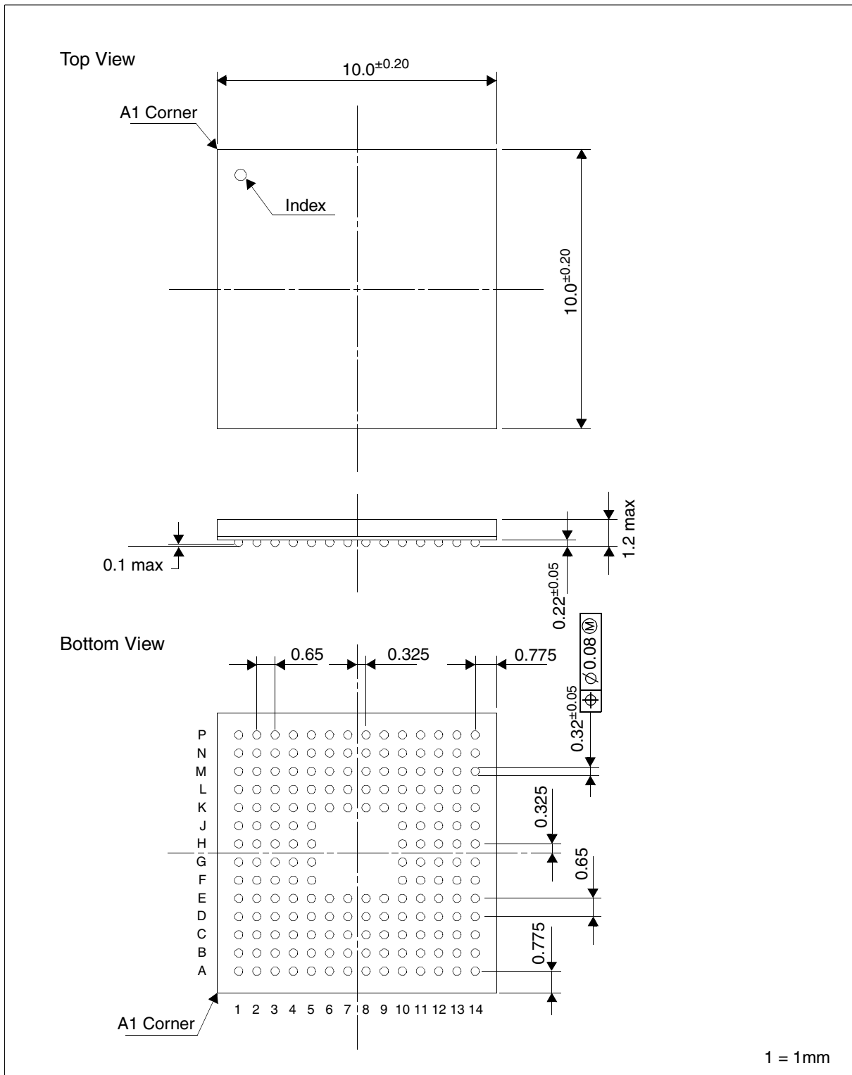
Figure 24-1: S1D13719 PFBGA 180-pin Package
