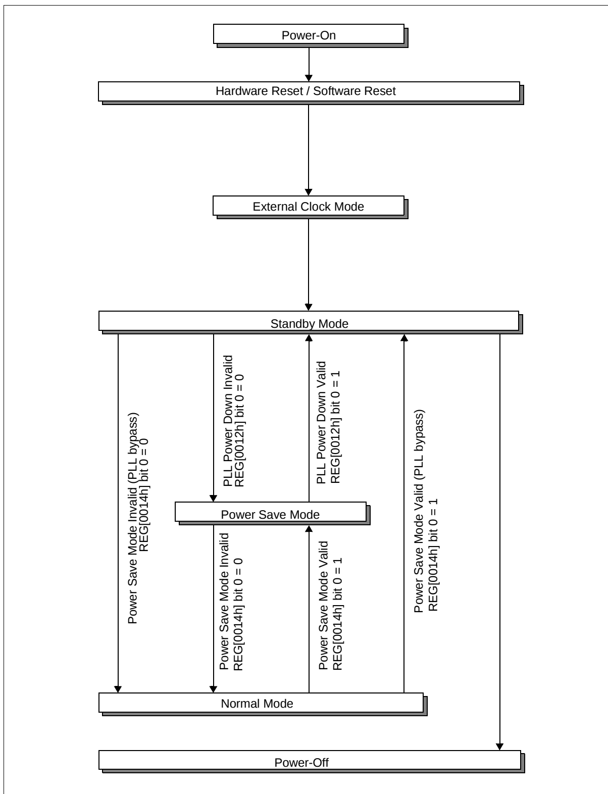
Figure 11-2: Power Modes
