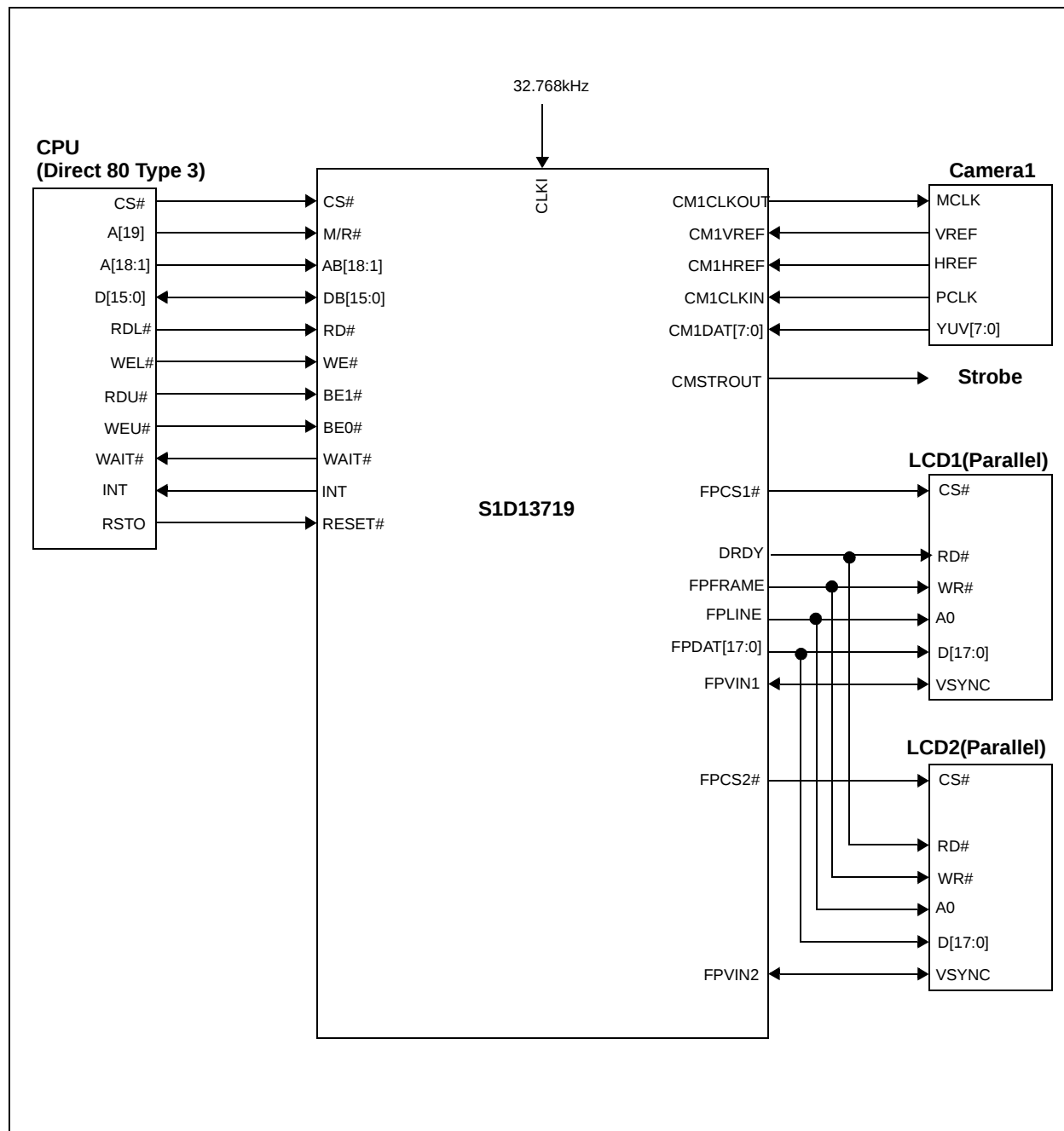
Figure 3-3: Example System Diagram 3
