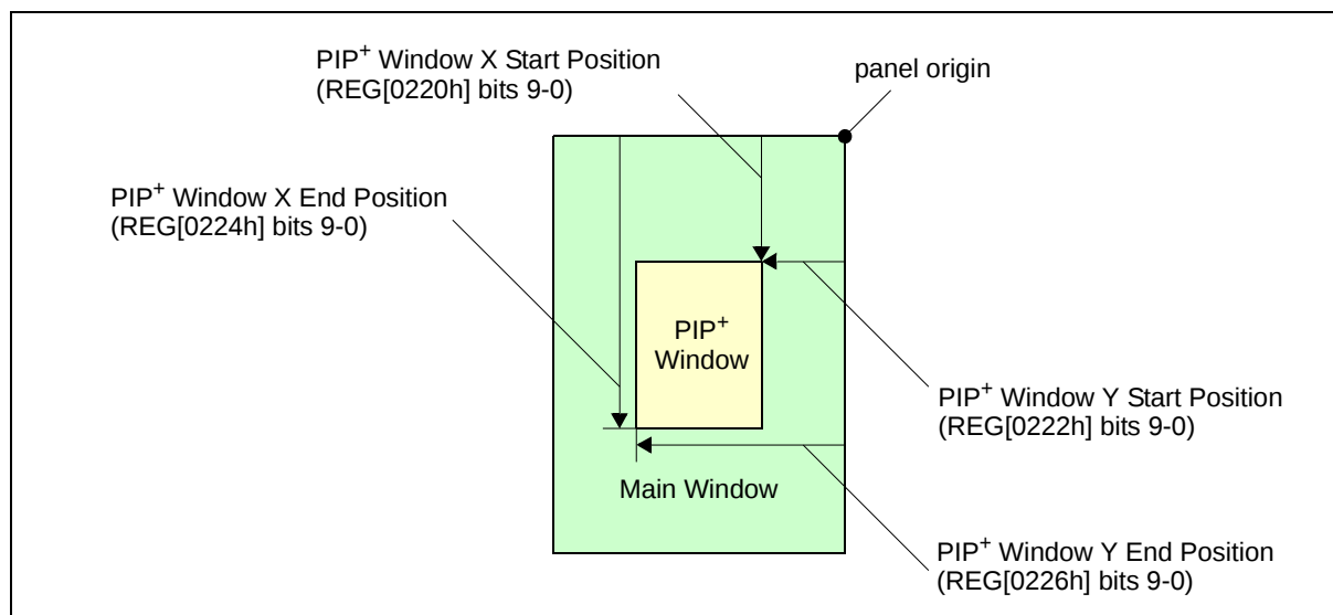
Figure 13-9: PIP + Window in SwivelView 90° Main Window
