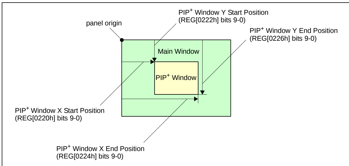
Figure 13-8: PIP + Display
