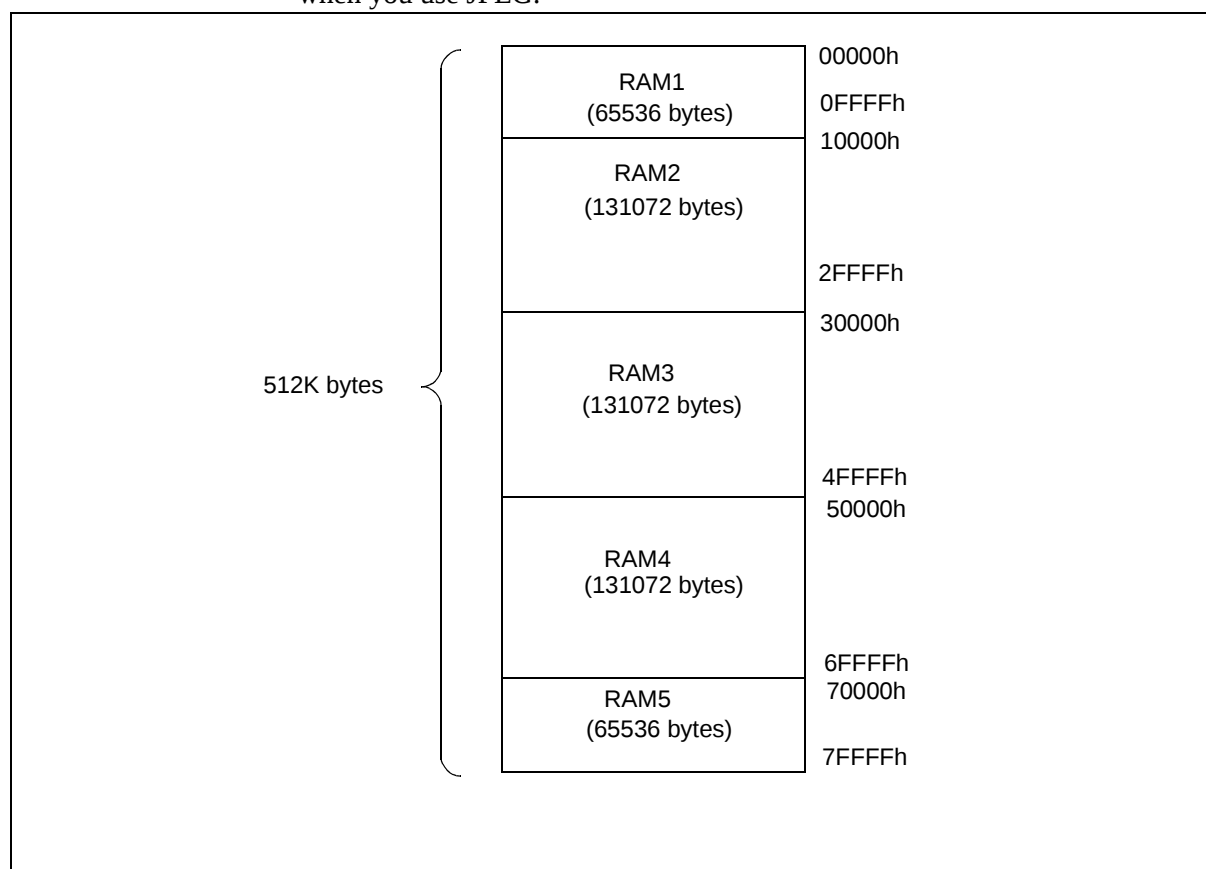
Figure 8-1: Physical Memory
