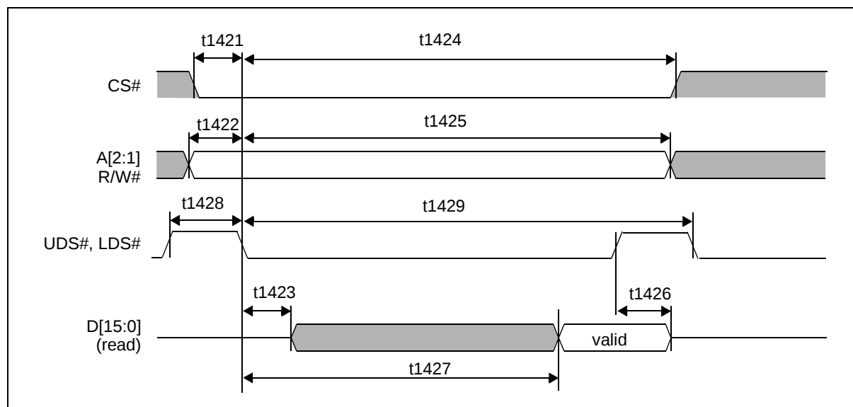
Figure 7-21: Indirect 68 Interface Read Cycle Timing
