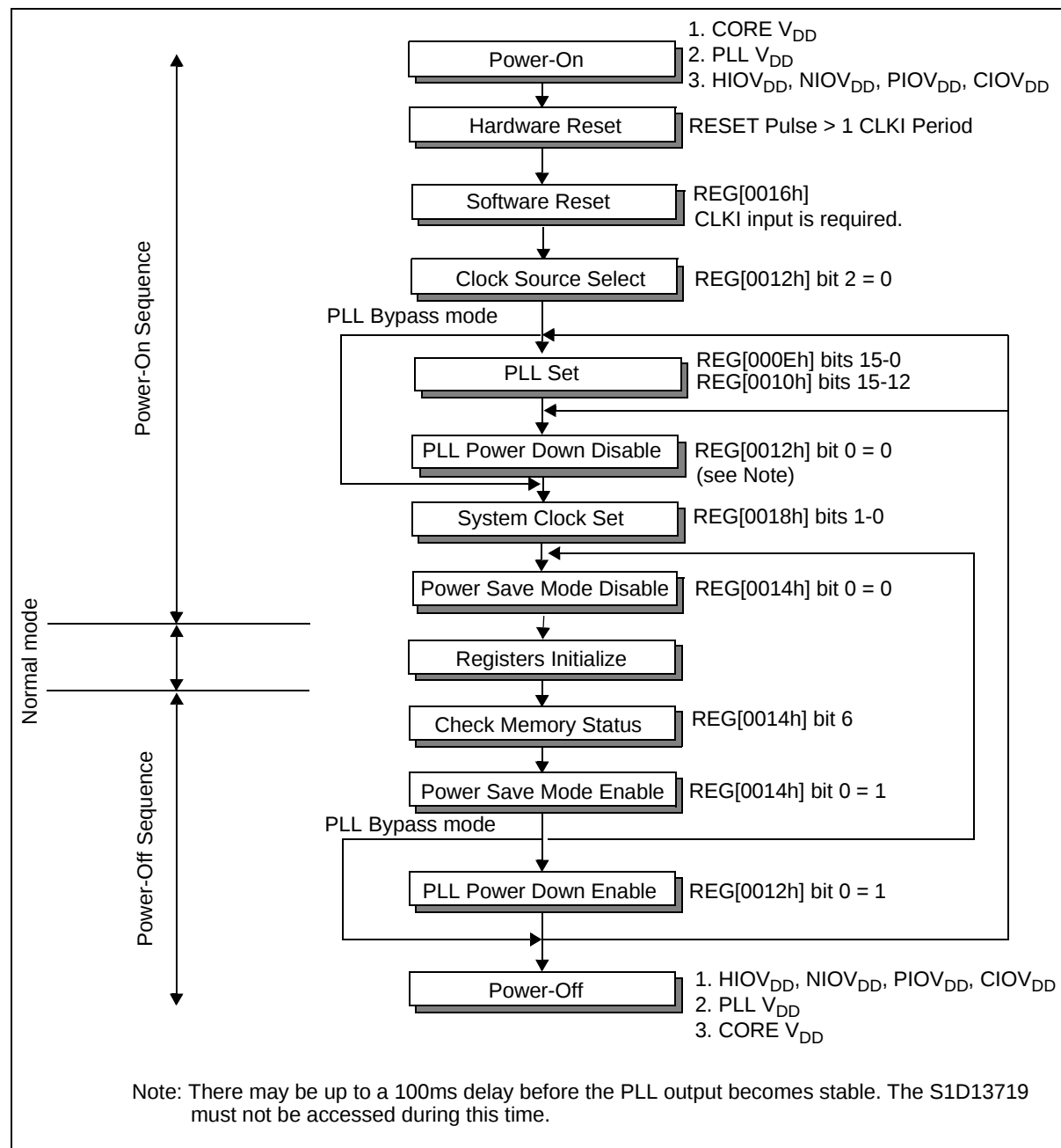
Figure 11-1: Power-On/Power-Off Sequence
