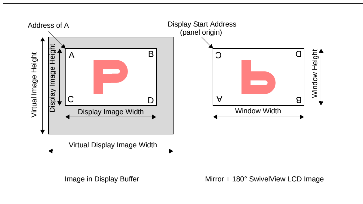
Figure 13-6: Mirror and 180° SwivelView Display
