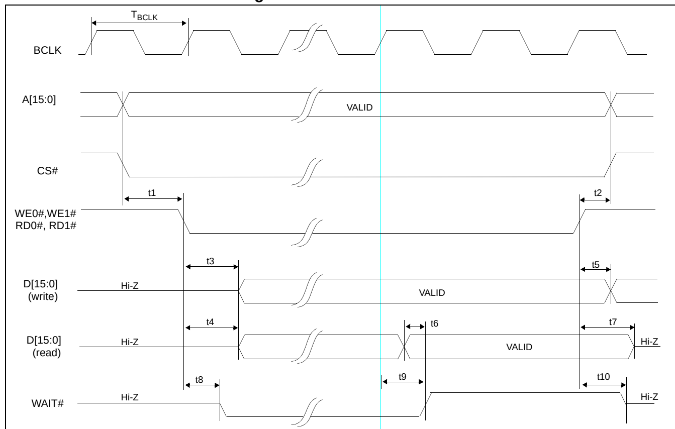
Figure 7-5: Generic #1 Timing
