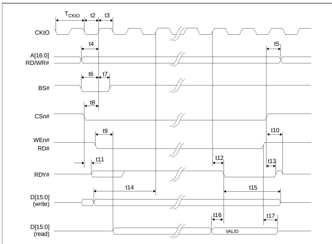
Figure 7-1: SH-4 Timing
