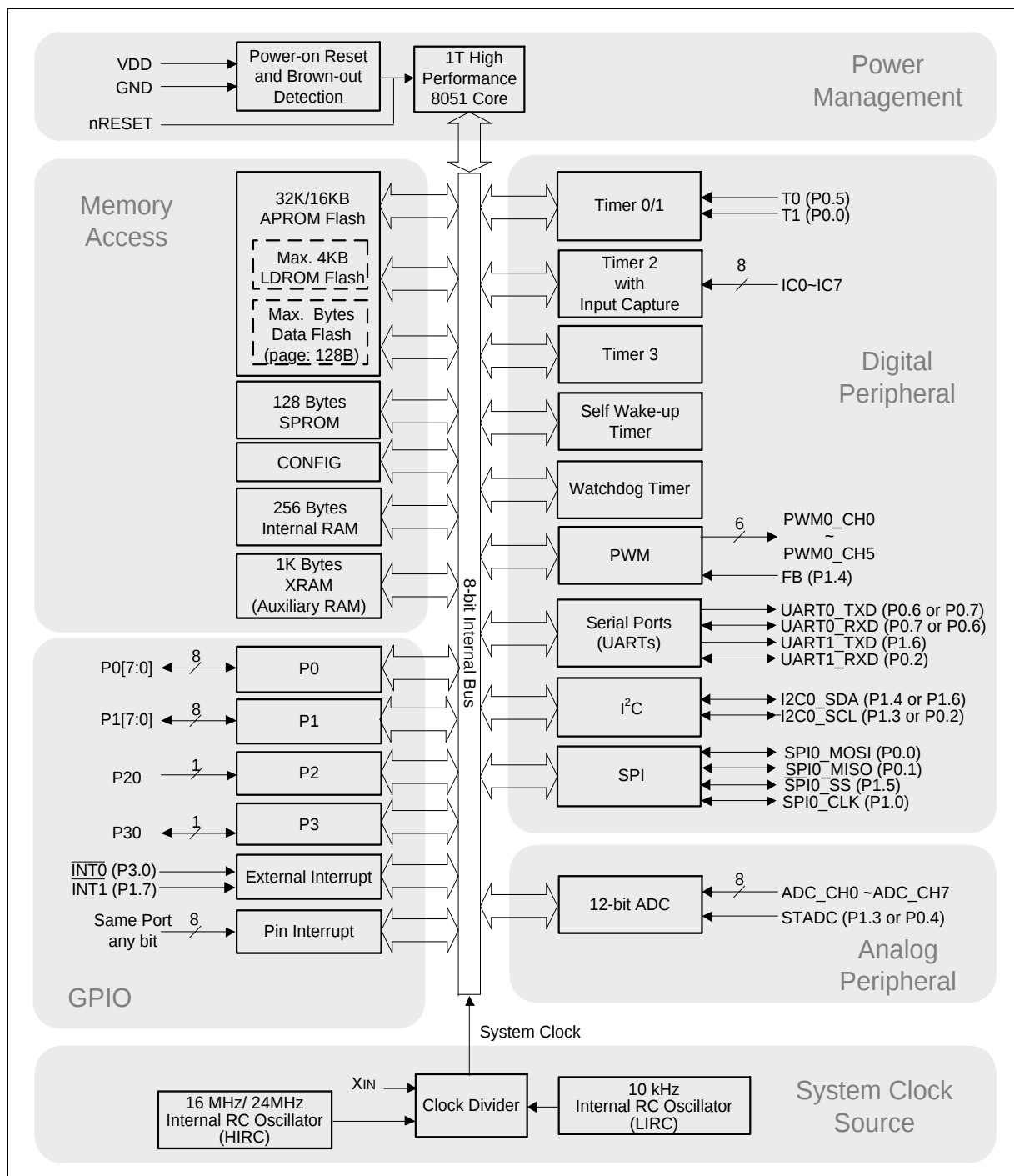
Figure 5.1-1 MG51 Series Functional Block Diagram
