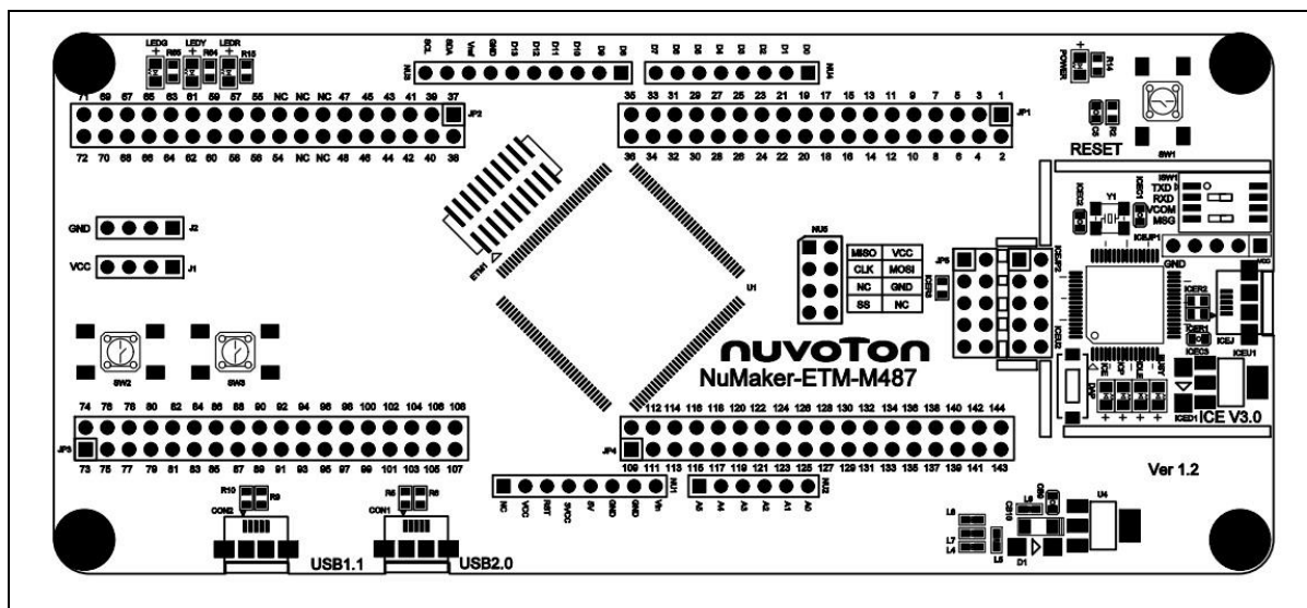
Figure 2-4 Front Placement
