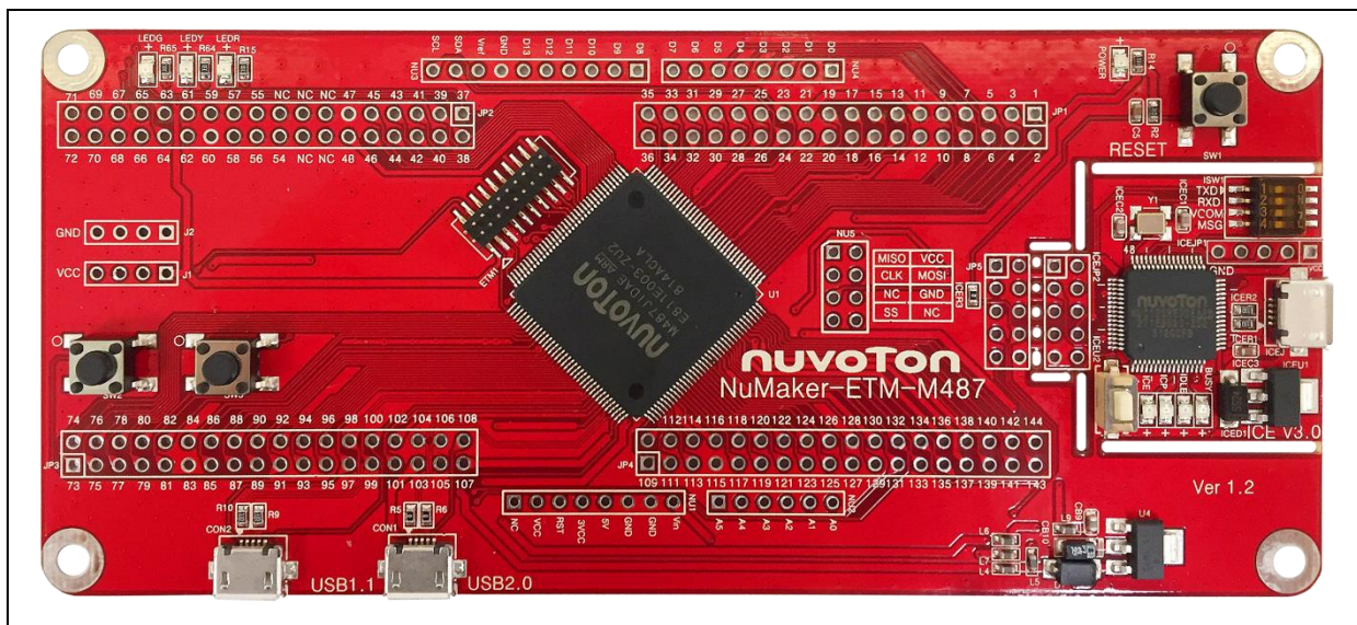
Figure 1-1 NuMaker-ETM-M487 Board
