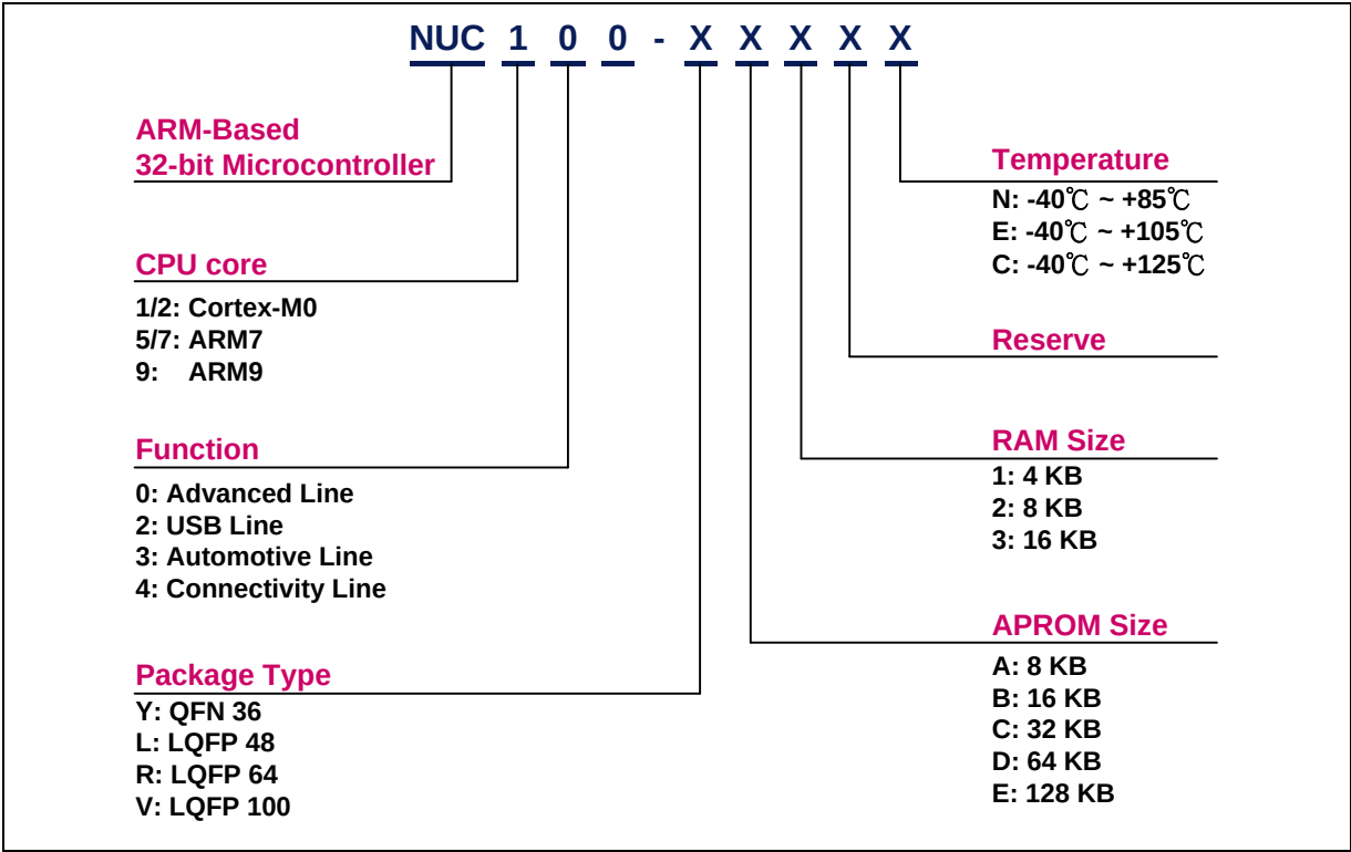
Figure 4-1 NuMicro® NUC100 Series Selection Code
