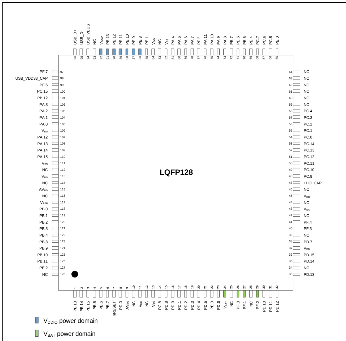
Figure 4.3-3 NuMicro® NUC029KGE LQFP 128-pin Diagram
