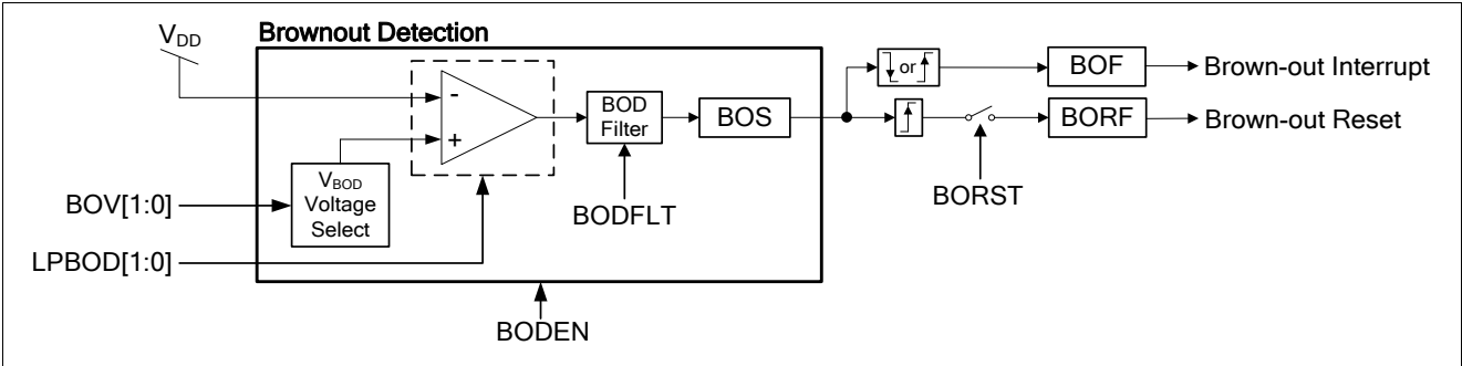
Figure 24.2-1. Brown-out Detection Block Diagram
