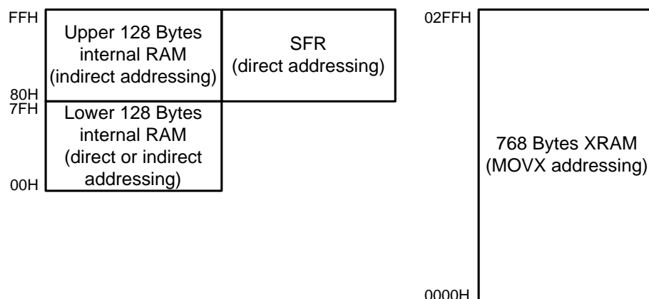
Figure 5.2-1. Data Memory Map
