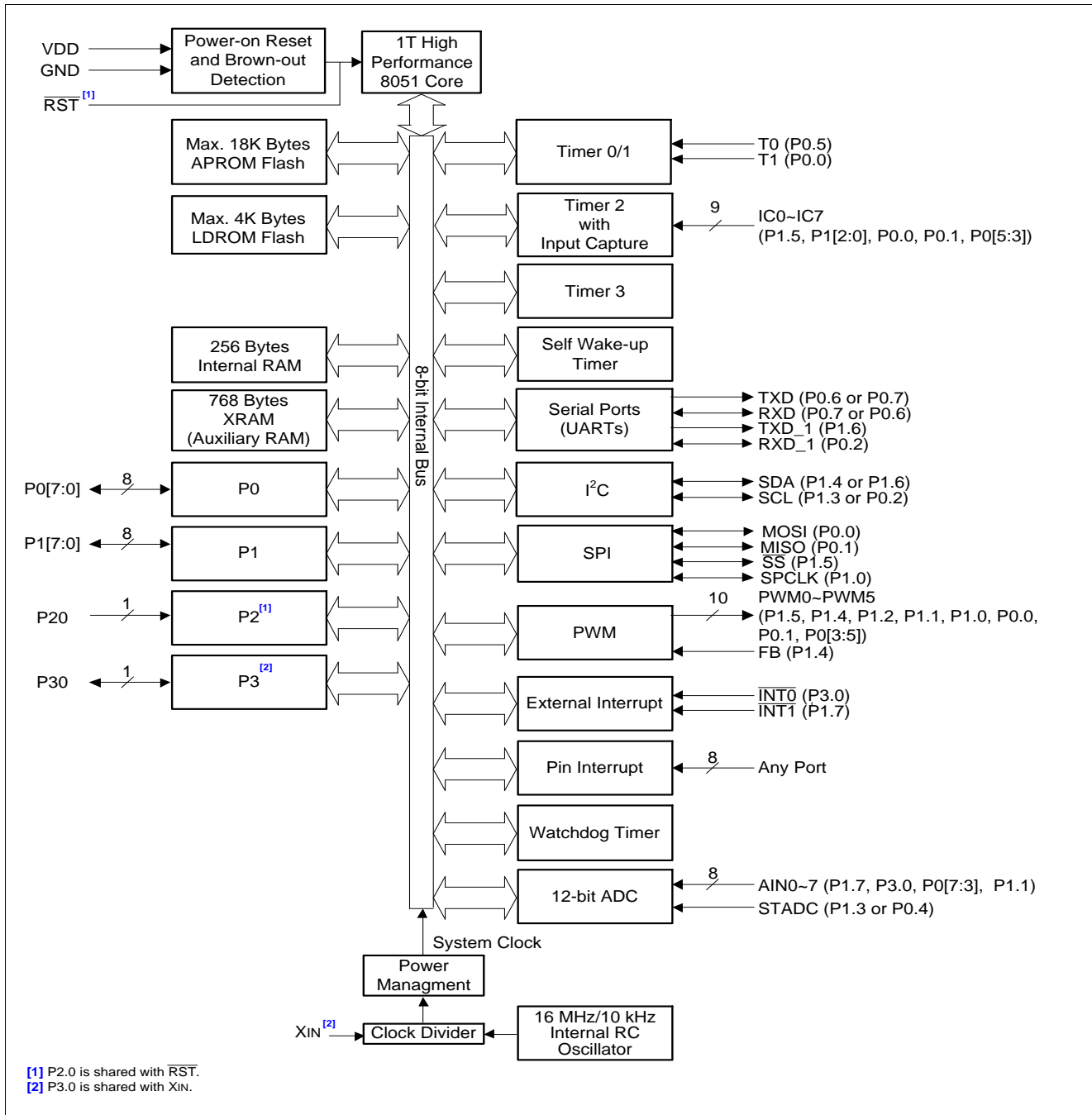
Figure 5.1-1. Functional Block Diagram
