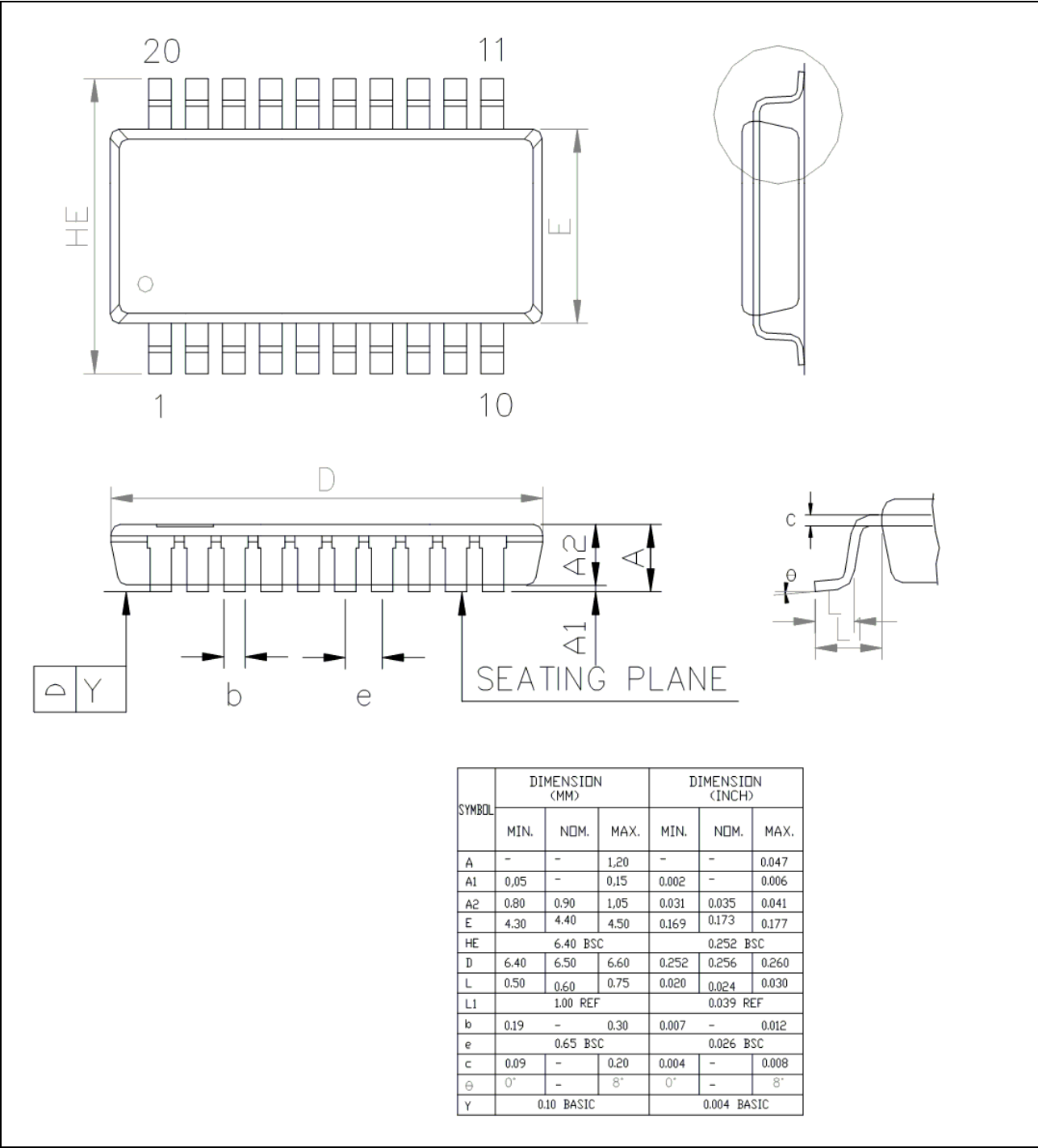
Figure 32.1-1. TSSOP-20 Package Dimension
