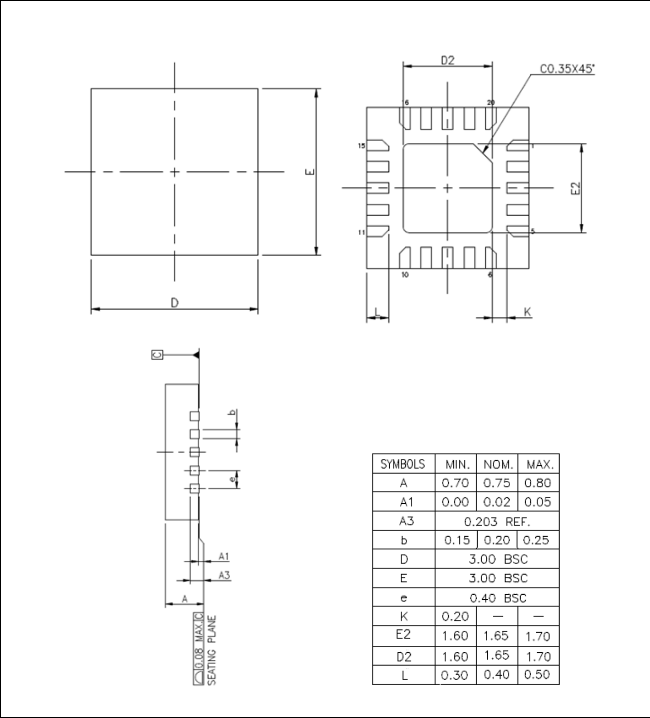
Figure 32.3-1. QFN-20 Package Dimension of N76E003AQ20
