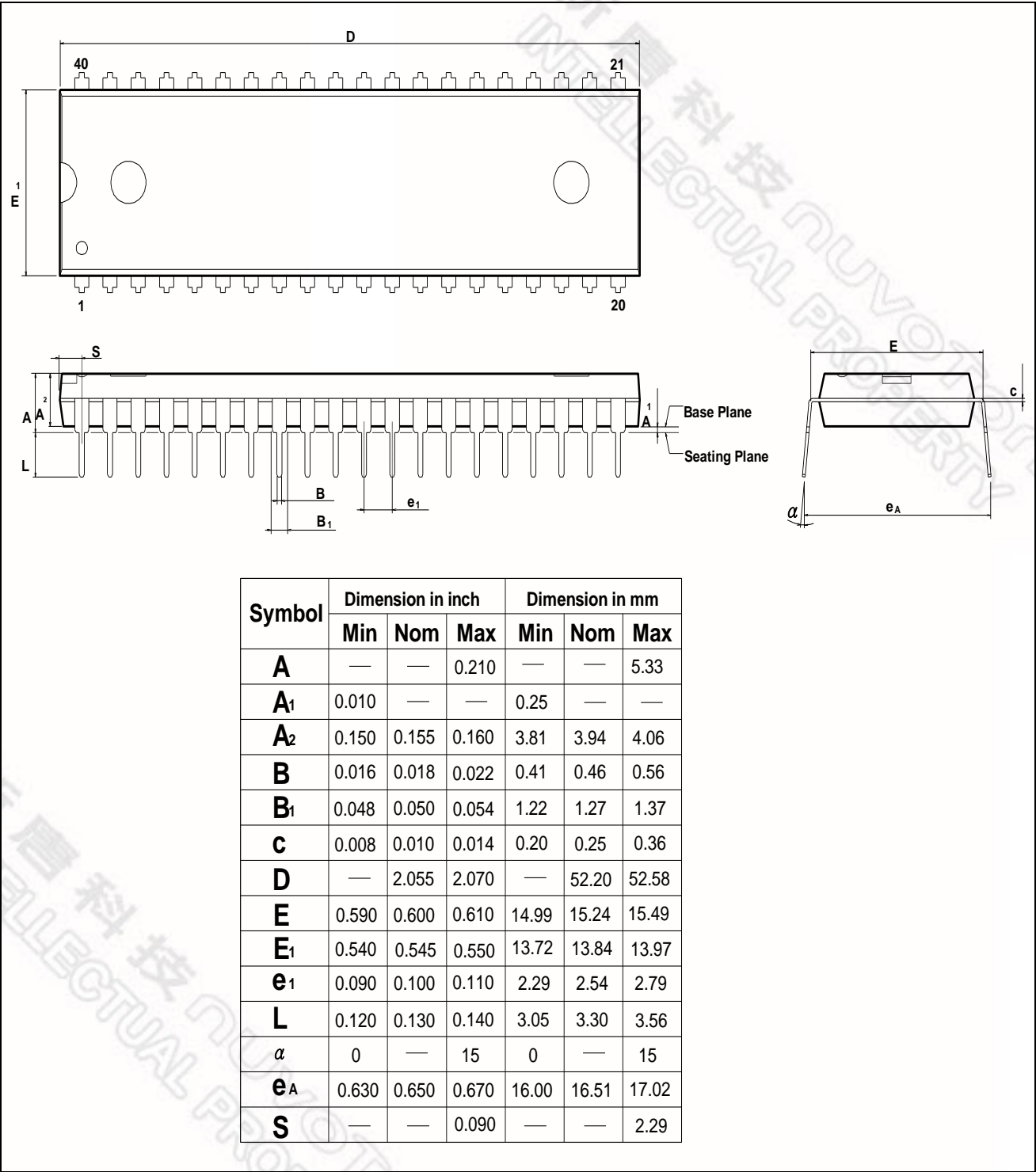
Figure 27-1. DIP-40 Package Dimention
