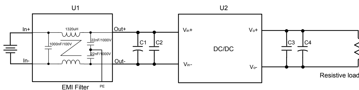
Figure 16 EMC test configuration
