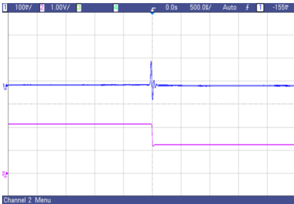
Fig.32 AVO50-48S1V8 typical transient response to step decrease in load from 50% to 25% of full load, room temperature, 48Vdc input ( \Delta I_o/\Delta t = 1A/1\mu s )
