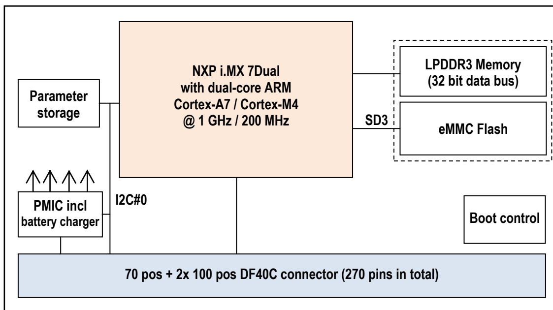
Figure 1 – iMX7 Dual uCOM Board Block Diagram
