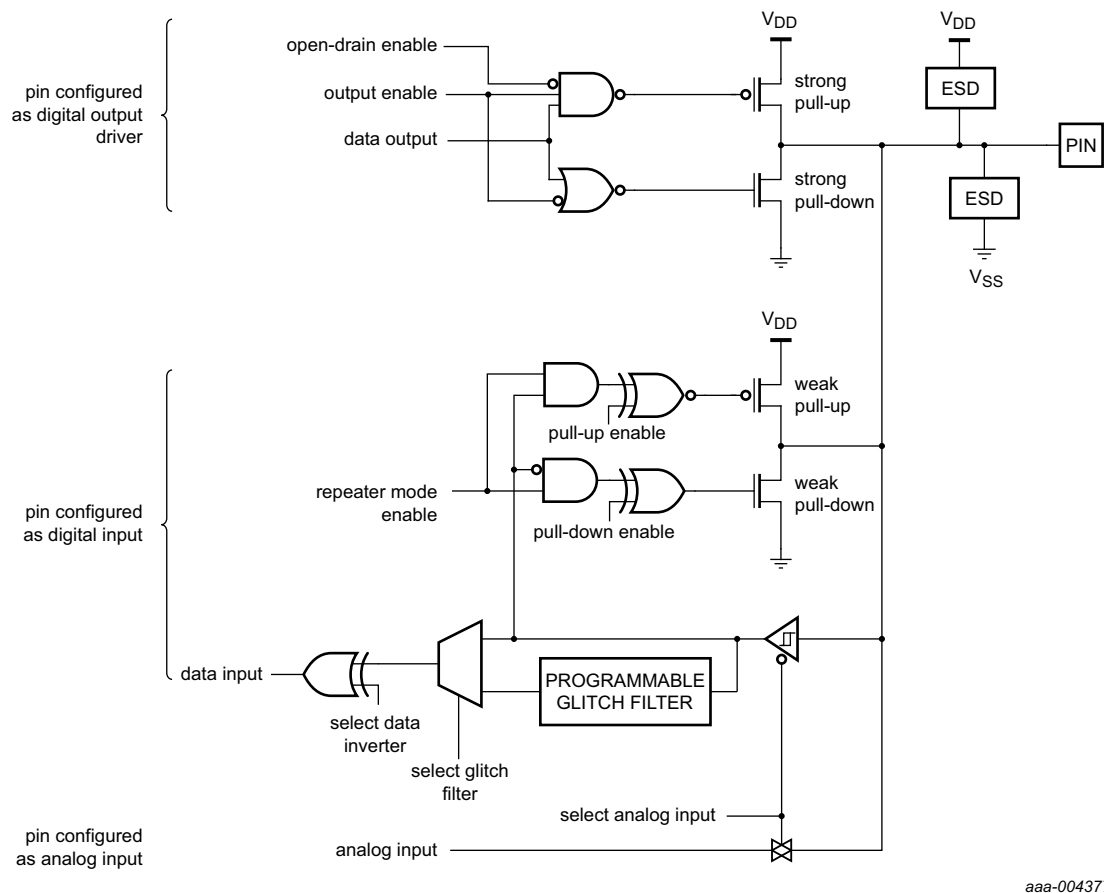
Fig 8. Standard I/O pad configuration
