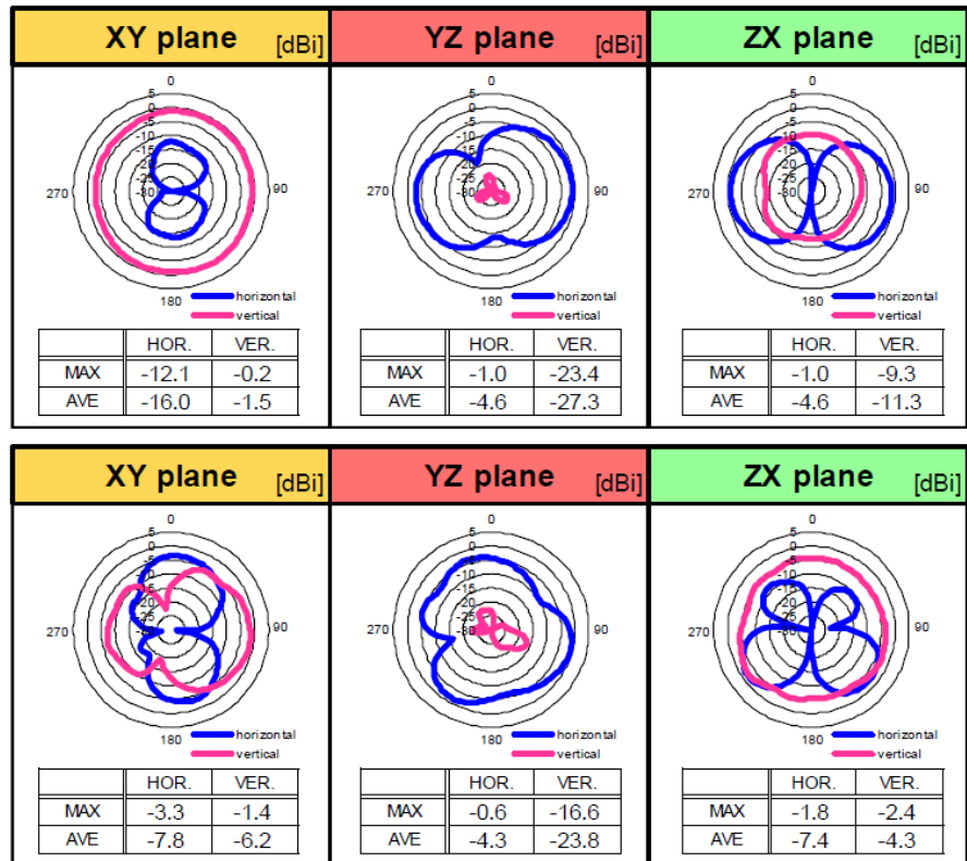
Figure 15 – Directivity for 1LV M.2 Module Standalone
