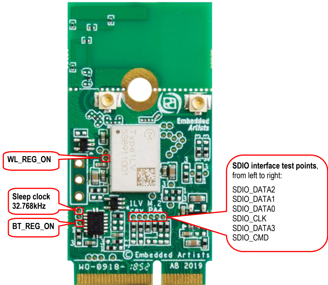
Figure 4 – 1LV M.2 Module Test Points
