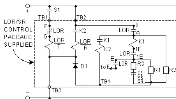
Fig. 6. Time-delay Self-reset circuit for the LOR/SR
