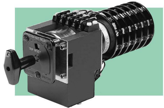
Fig. 2. Series 24 LOR/ER Electric-reset Lock-out Relay and LOR/SR Self-reset Lock-out Relay
