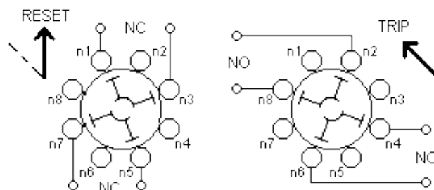
Fig. 14. Basic LOR Deck Layout
