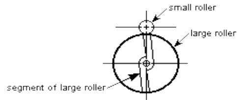
Fig. 16. Relationship of two rollers with coincident radii
