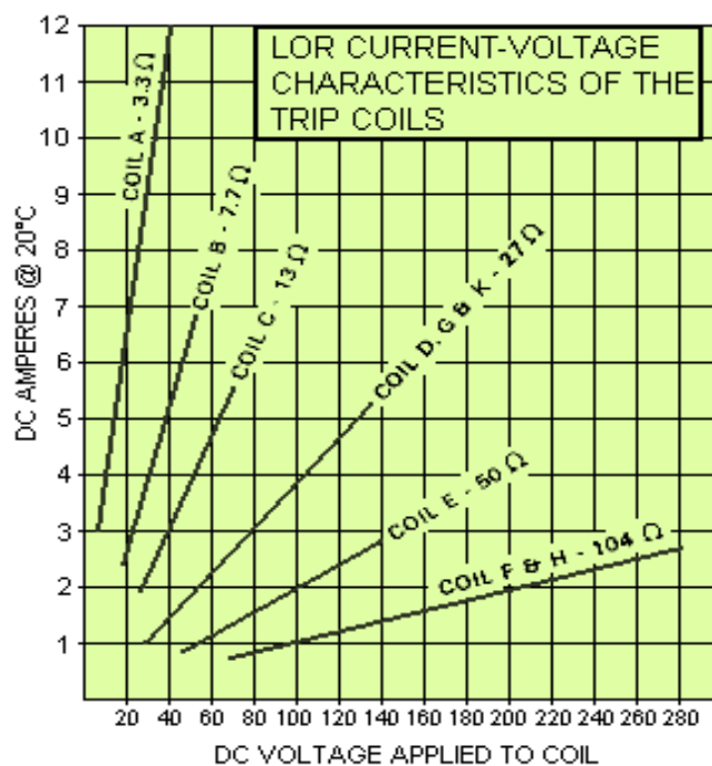
Fig. 7. Trip Solenoid Coil Burden Data
