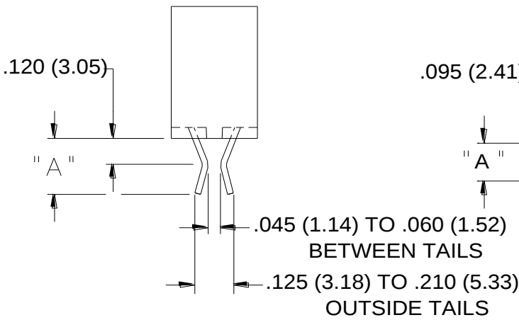
CONTACT CODE 555 BEND USES WIRE HOLE CONTACTS
