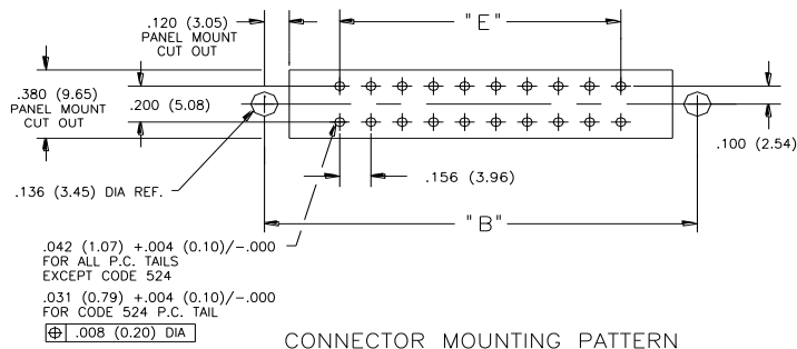
CONNECTOR MOUNTING PATTERN
