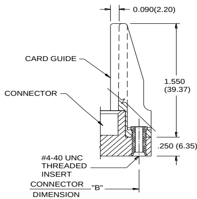
MOUNTING OPTION CODE x178 (IN-LINE CARD GUIDE)
