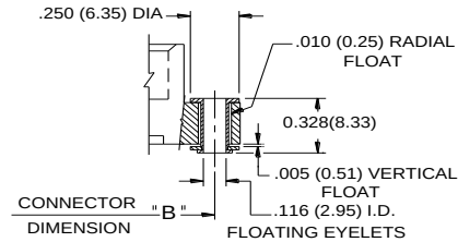
MOUNTING OPTION CODE x103 (FLOATING EYELETS)
