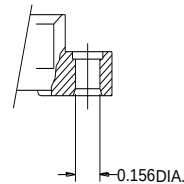
VARIATION 04 .156±.002 DIA. MOUNTING HOLE
