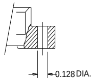
VARIATION 02 .128±.003 DIA. MOUNTING HOLE
