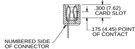
SINGLE ROW CONTACTS READ BOTH SIDES OF DAUGHTER BOARD
