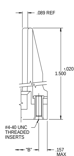
MOUNTING OPTION CODE #78
