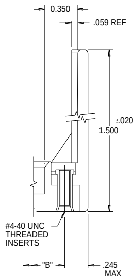
MOUNTING OPTION CODE #68
