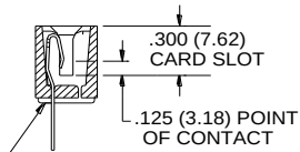
SINGLE ROW CONTACTS READ ONE SIDE OF DAUGHTER BOARD
