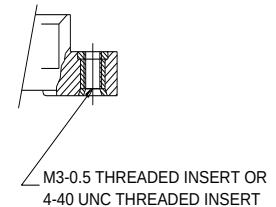
VARIATIONS 07 AND 08 THREADED INSERT
