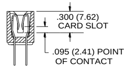
DUAL ROW CONTACTS
