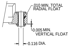
VARIATION 03 .116±.003 I.D. FLOATING EYELET
