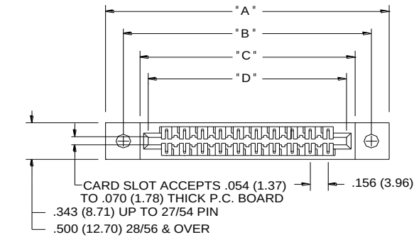
DUAL ROW CONTACTS
