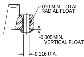
VARIATION 03 .116±.003 I.D. FLOATING EYELET -.000
