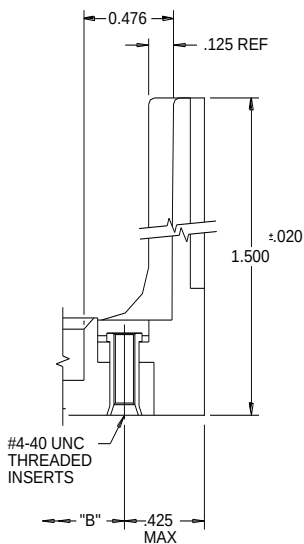
MOUNTING OPTION CODE #58
