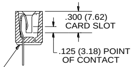
SINGLE ROW CONTACTS READ ONE SIDE OF DAUGHTER BOARD
