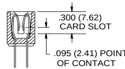
DUAL ROW CONTACTS
