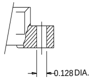
VARIATION 02 .128±.003 DIA. MOUNTING HOLE
