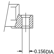
VARIATION 04 .156±.002 DIA. MOUNTING HOLE -.000
