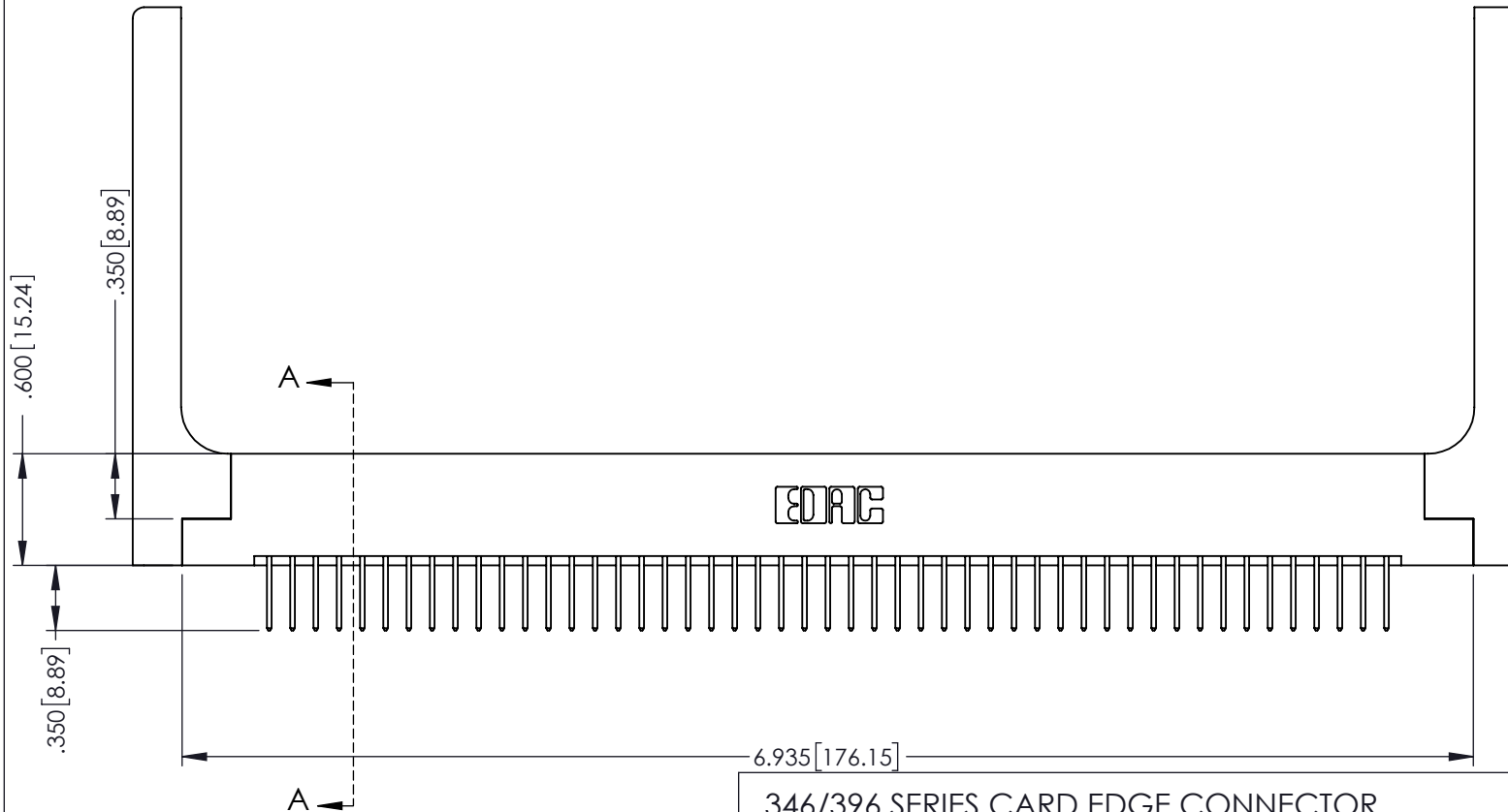
• INSULATOR MATERIAL: THERMOPLASTIC POLYESTER, UL 94V-0 • CONTACT MATERIAL: COPPER, NICKEL, TIN ALLOY CA-725 • CONTACT PLATING: GOLD ON THE MATING AREA, TIN-LEAD ON THE CONTACT TAILS, NICKEL UNDERPLATE
