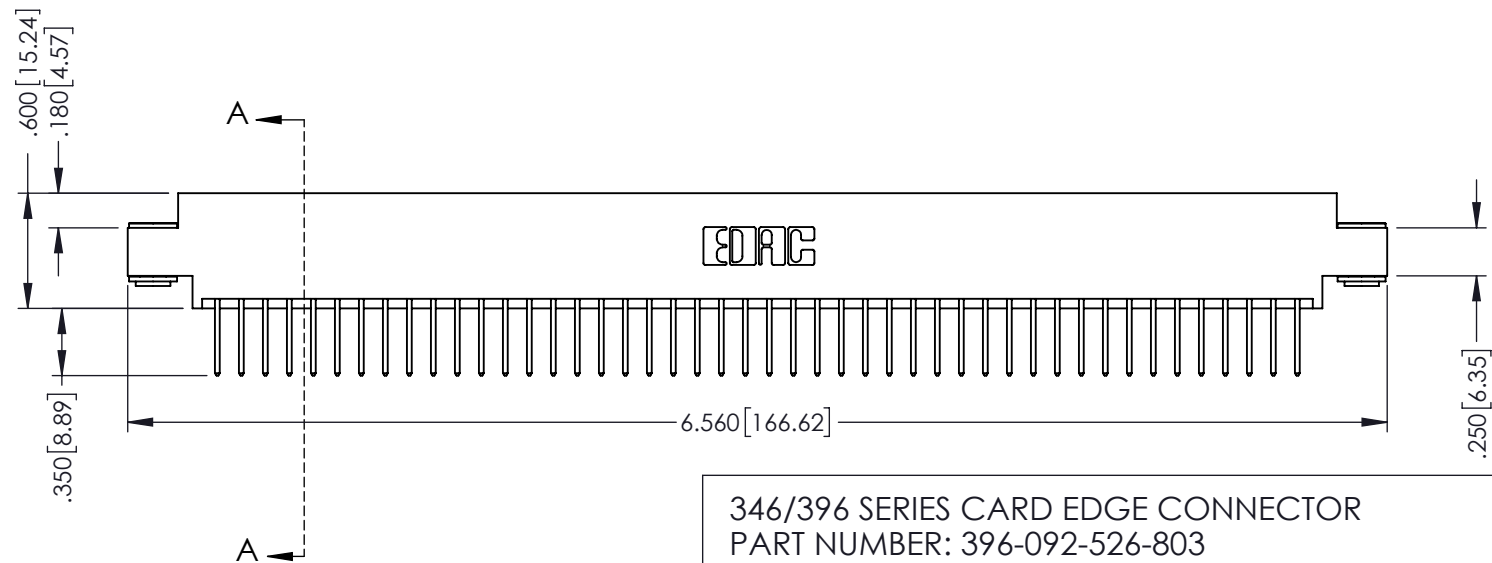
• INSULATOR MATERIAL: THERMOPLASTIC POLYESTER, UL 94V-0 • CONTACT MATERIAL: COPPER, NICKEL, TIN ALLOY CA-725 • CONTACT PLATING: GOLD ON THE MATING AREA, TIN-LEAD ON THE CONTACT TAILS, NICKEL UNDERPLATE
