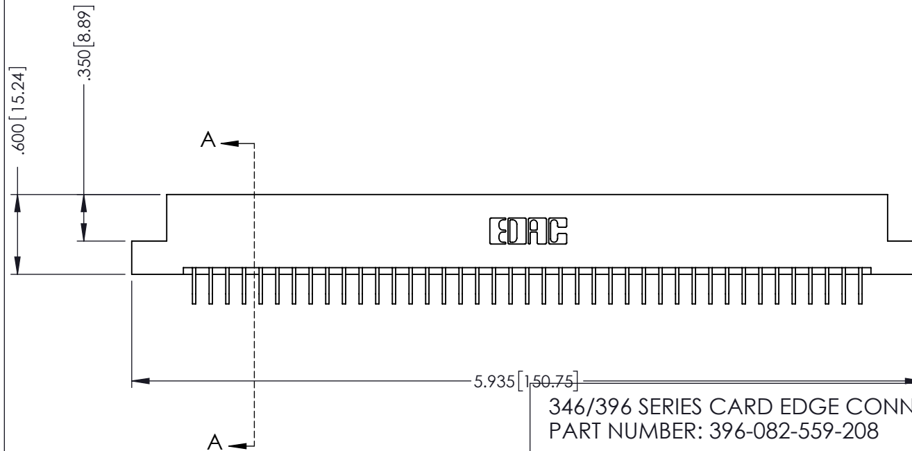
• INSULATOR MATERIAL: THERMOPLASTIC POLYESTER, UL 94V-0 • CONTACT MATERIAL: COPPER, NICKEL, TIN ALLOY CA-725 • CONTACT PLATING: GOLD ON THE MATING AREA, TIN-LEAD ON THE CONTACT TAILS, NICKEL UNDERPLATE
