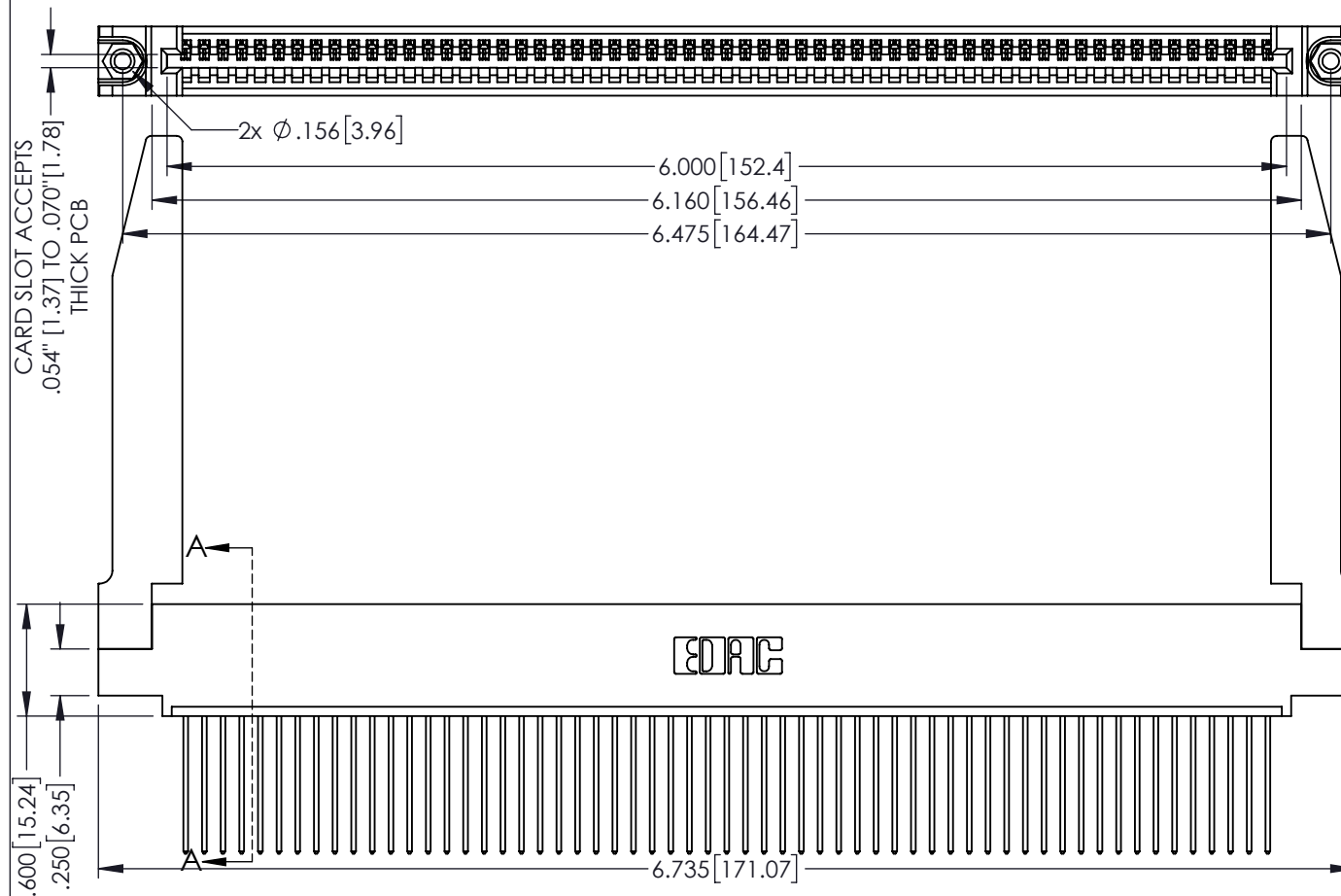
345/395 SERIES CARD EDGE CONNECTOR PART NUMBER: 395-059-541-478
