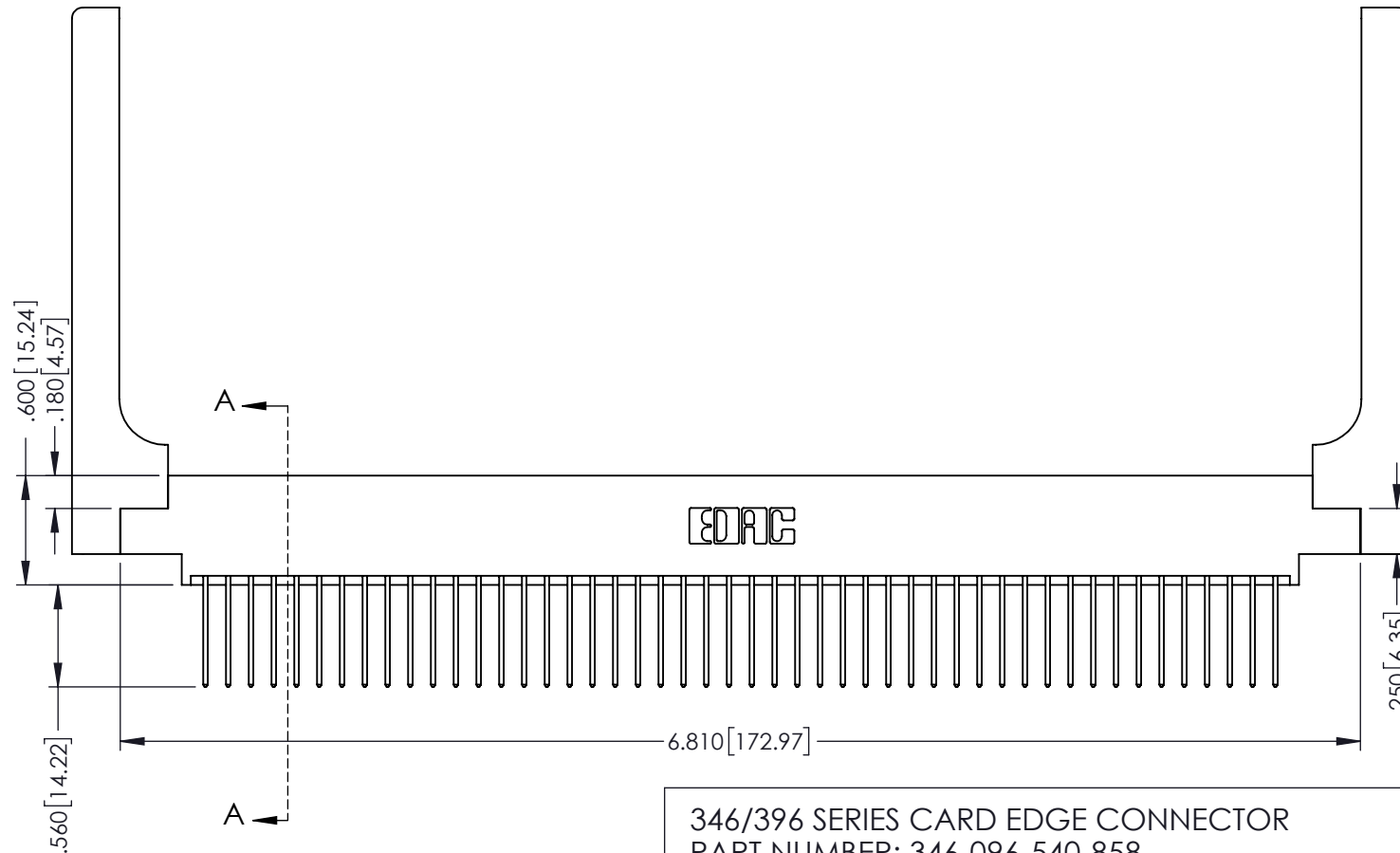
• INSULATOR MATERIAL: THERMOPLASTIC POLYESTER, UL 94V-0 • CONTACT MATERIAL: COPPER, NICKEL, TIN ALLOY CA-725 • CONTACT PLATING: GOLD ON THE MATING AREA, TIN-LEAD ON THE CONTACT TAILS, NICKEL UNDERPLATE
