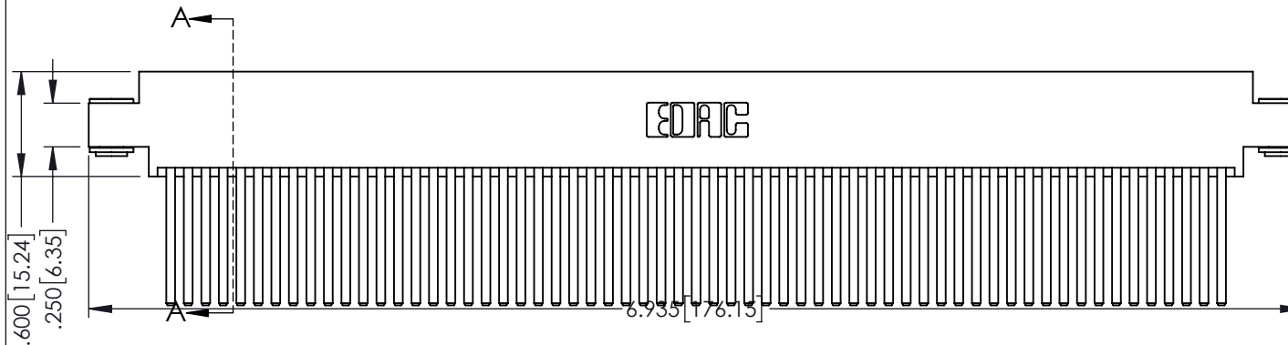
345/395 SERIES CARD EDGE CONNECTOR PART NUMBER: 345-122-544-803
