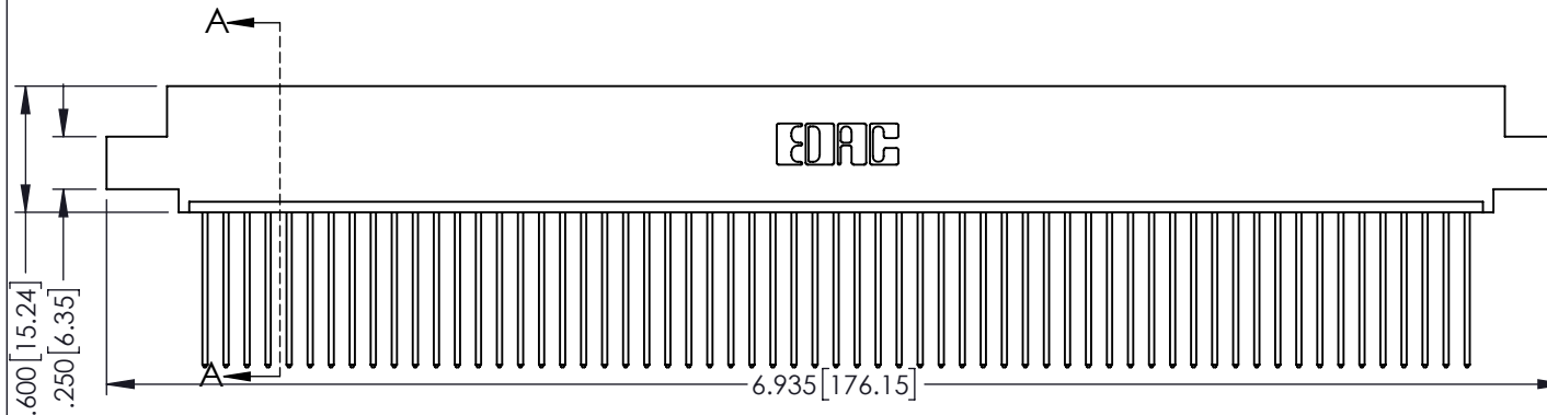
345/395 SERIES CARD EDGE CONNECTOR PART NUMBER: 345-061-541-404
