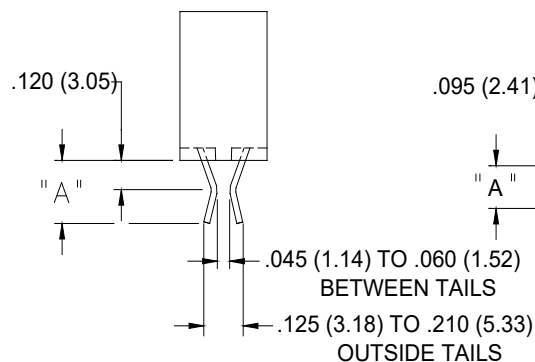
CONTACT CODE 555 BEND USES WIRE HOLE CONTACTS
